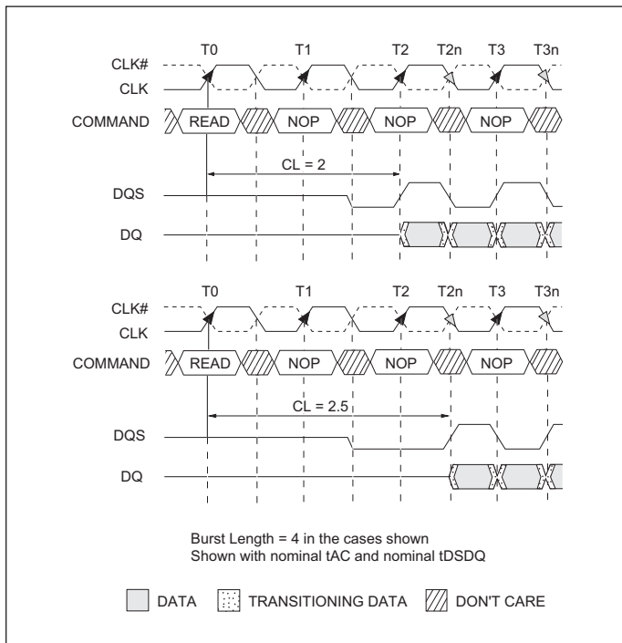
FIGURE 4 – CAS LATENCY
