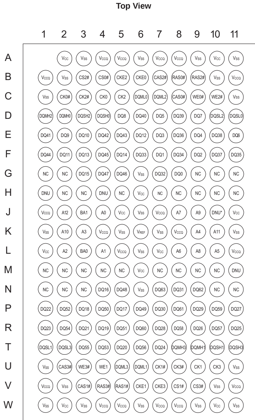
FIGURE 1 – PIN CONFIGURATION
