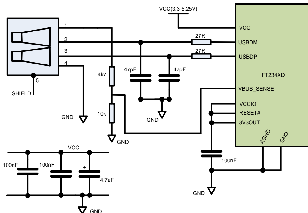
Figure 6.2 Self-Powered Configuration
