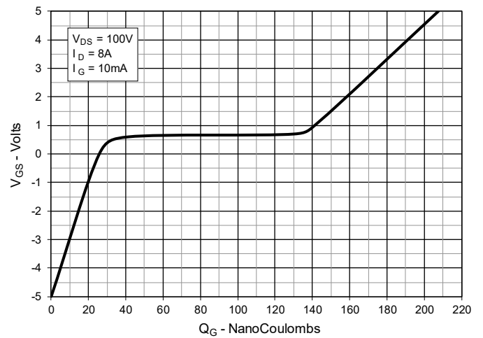
Fig. 14. Gate Charge
