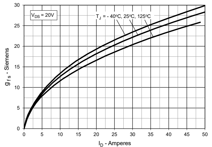
Fig. 10. Transconductance
