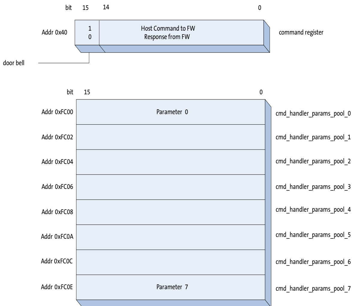
Figure 15: Interface Structure
