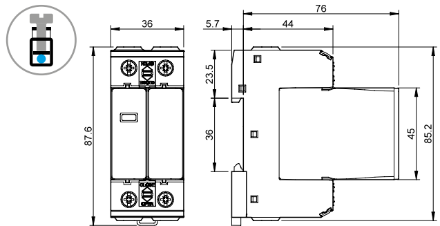
Type 7P02.8.275.1012 Box clamp
