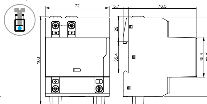
Type 7P.13.9.500.x006 Box clamp
