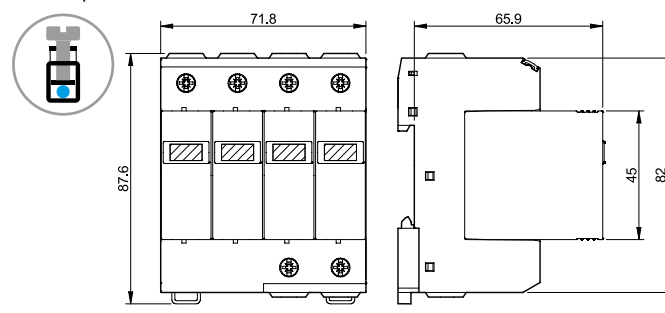
Types 7P.25/7P.45 Box clamp
