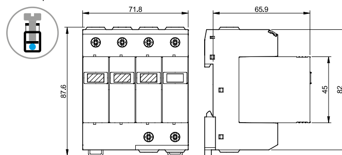
Types 7P.24/7P.44 Box clamp
