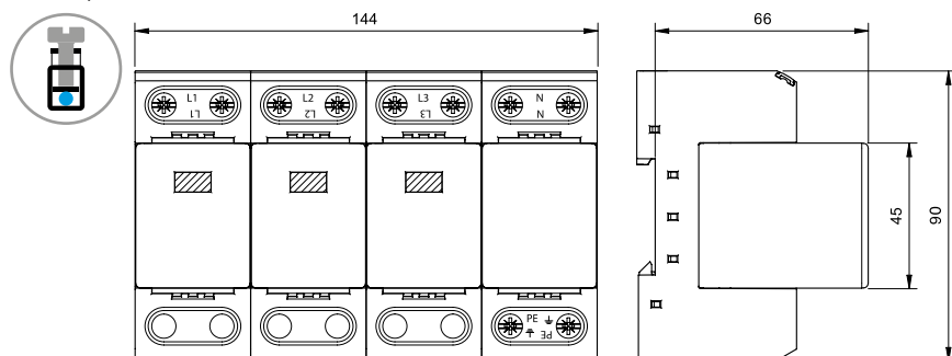
Type 7P.04 Box clamp
