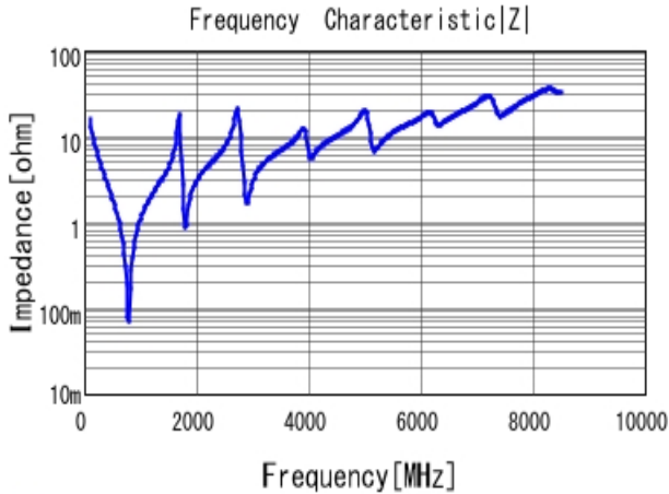
■ GQM2195C2E101JB12 |Z| DC0V, 25degC
