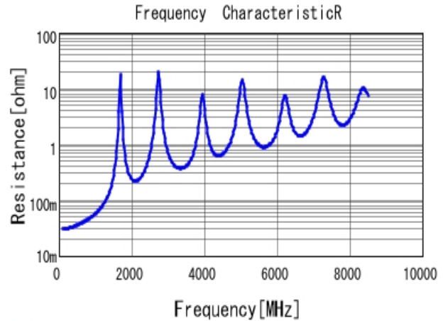
■ GQM2195C2E101JB12 R DC0V, 25degC
