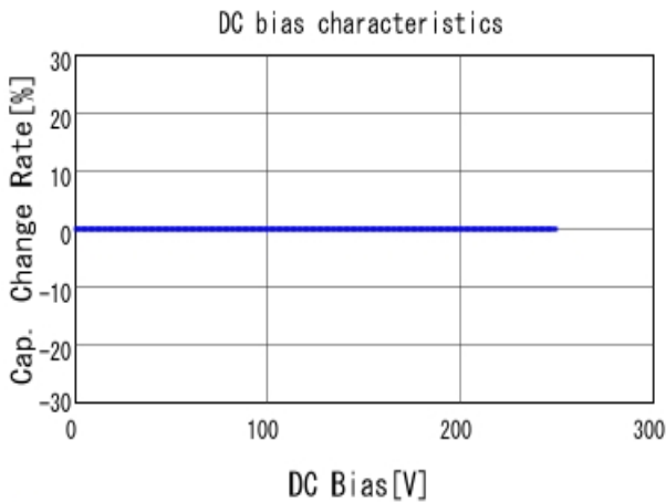
■ GQM2195C2E101JB12 C-DC bias capchange, 25.0degC, AC1V
