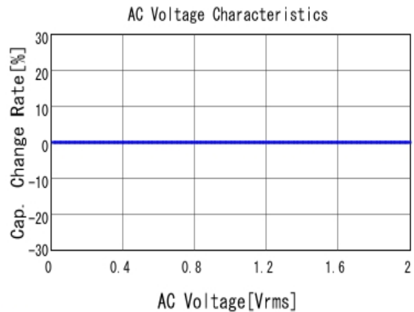
■ GQM2195C2E101JB12 C-AC Voltage capchange, DC0V, 25.0d
