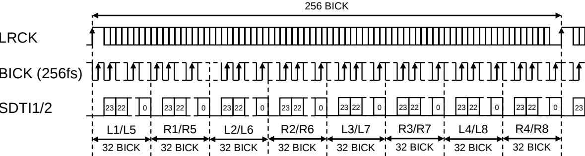
Figure 34. Mode 16 Timing
