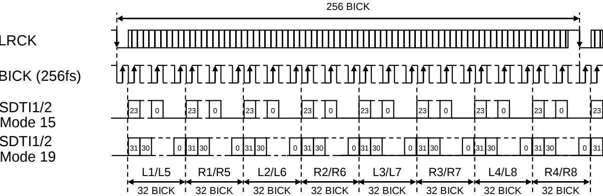
Figure 33. Mode 15/19 Timing
