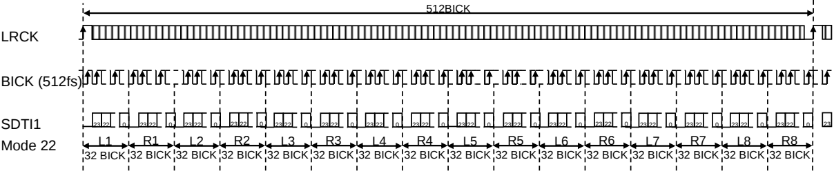
Figure 37. Mode 22 Timing
