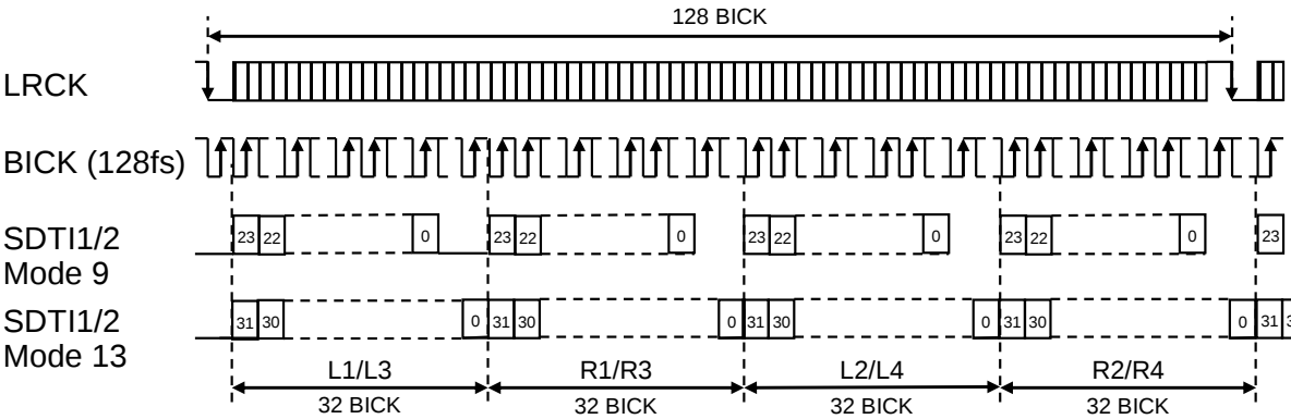
Figure 30. Mode 9/13 Timing
