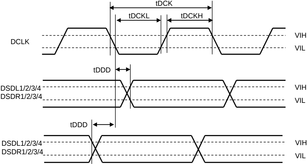
DSD Audio Interface Timing (DSD64/128/256 Mode)
