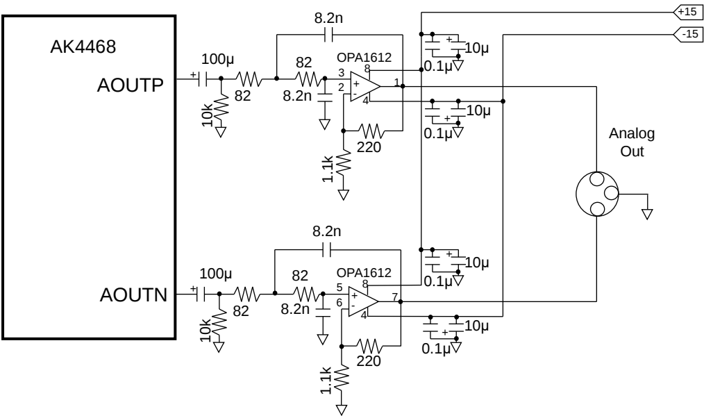
Figure 78. External LPF Circuit Example 3 (fc = 174 kHz (Typ), Q = 0.5 (Typ))
