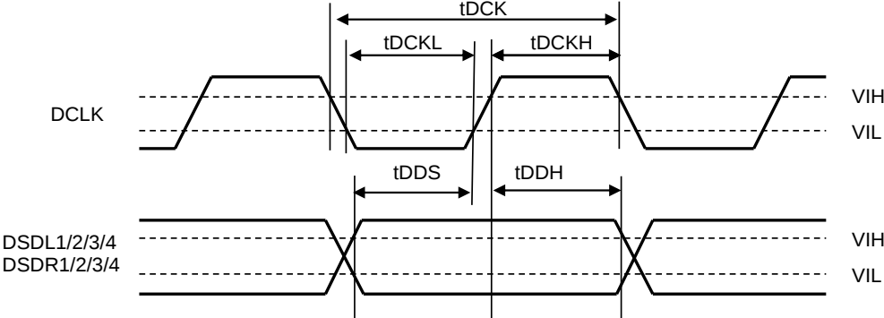
DSD Audio Interface Timing (DSD512 Mode)
