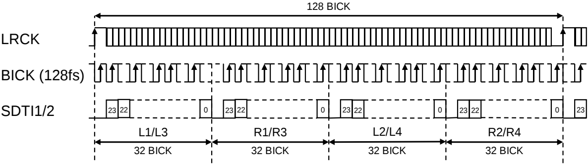
Figure 31. Mode 10 Timing
