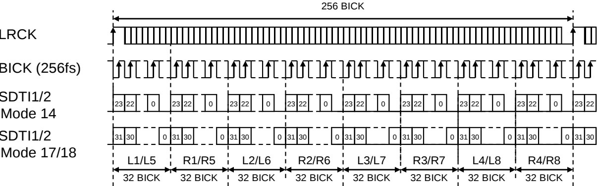
Figure 32. Mode 14/17/18 Timing
