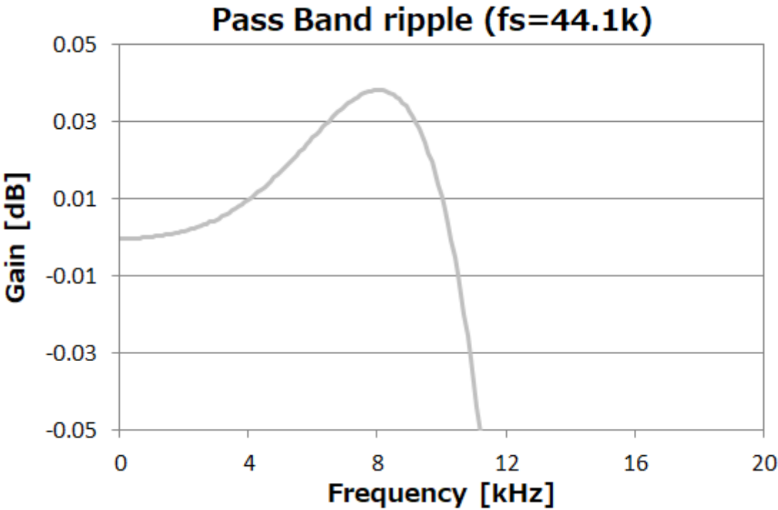
Figure 9. Short-delay Slow Roll-off Filter Passband Ripple
