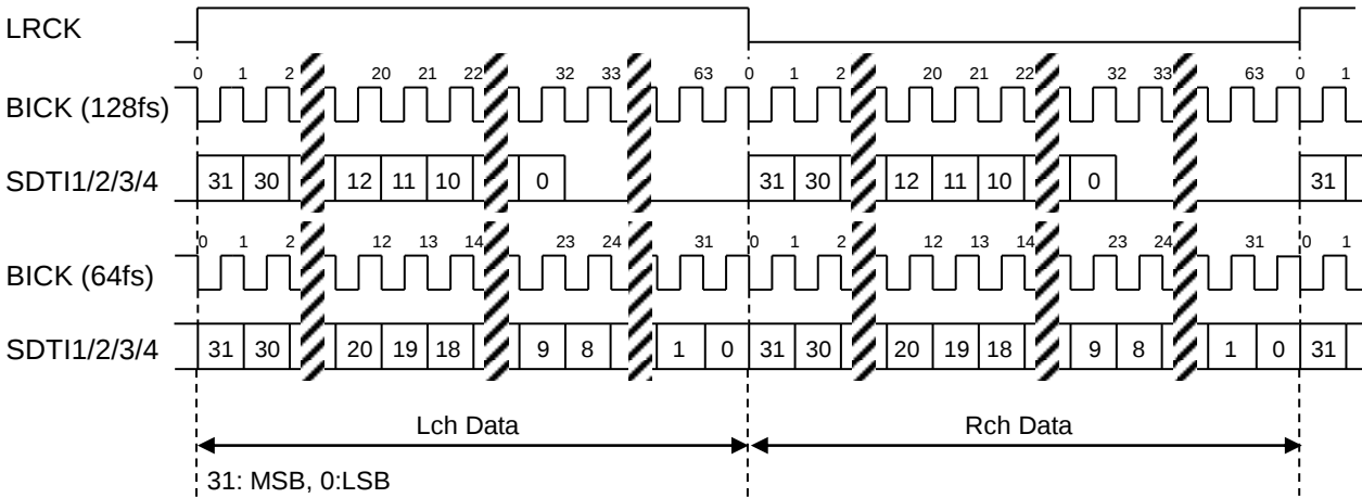
Figure 27. Mode 6 Timing
