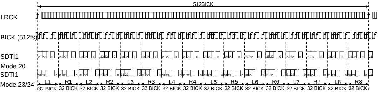
Figure 35. Mode 20/23/24 Timing
