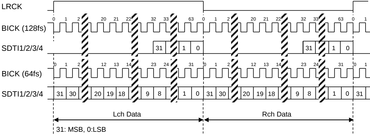
Figure 26. Mode 5 Timing
