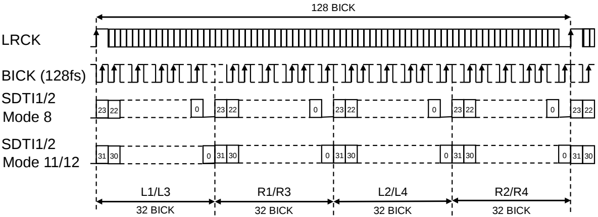
Figure 29. Mode 8/11/12 Timing
