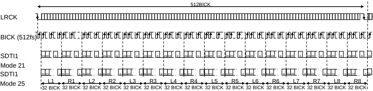
Figure 36. Mode 21/25 Timing
