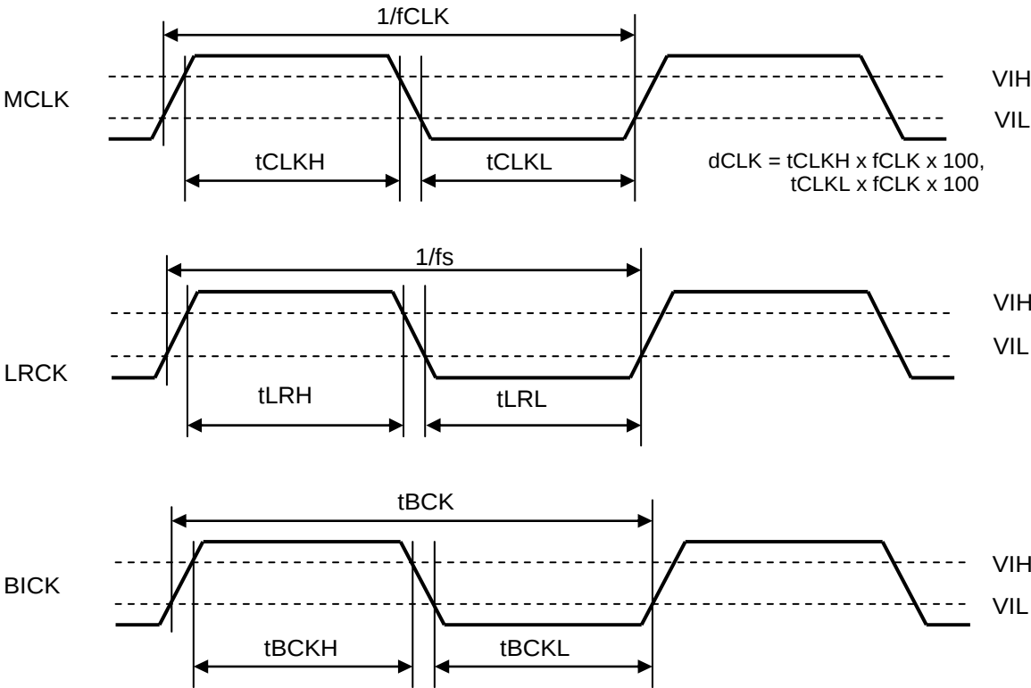
Figure 12. Clock Timing
