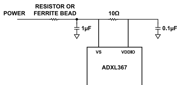
Figure 61. Recommended Decoupling Schematics for Single Supply
