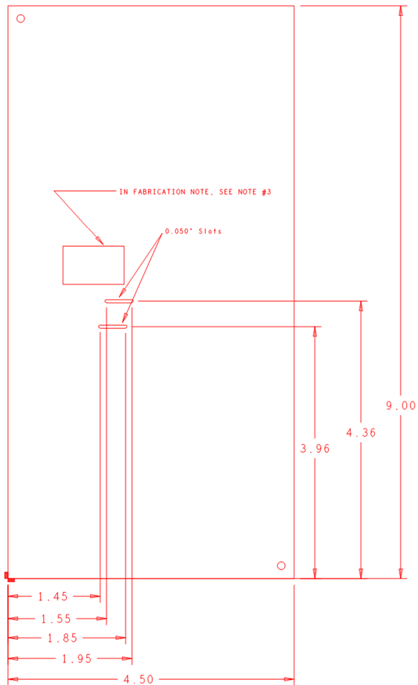
FIGURE 7 Circuit Outline
