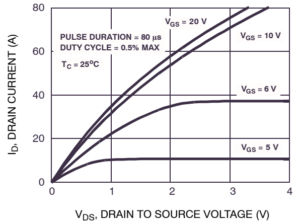
Figure 8. Saturation Characteristics
