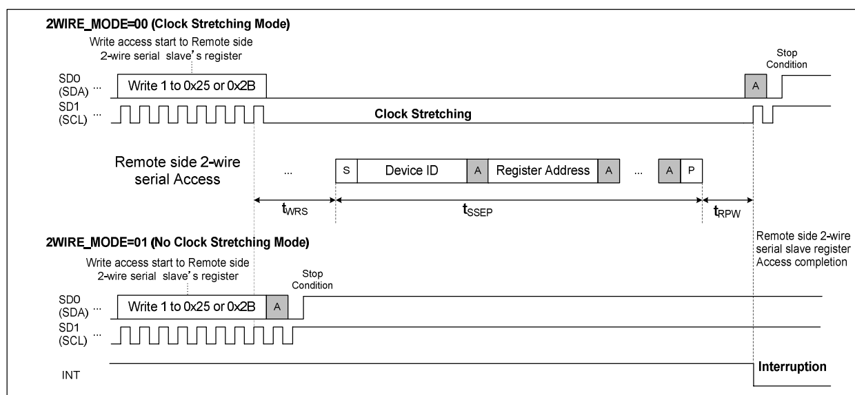
Figure 32. Write access completion time to Remote side 2-wire serial slave register
