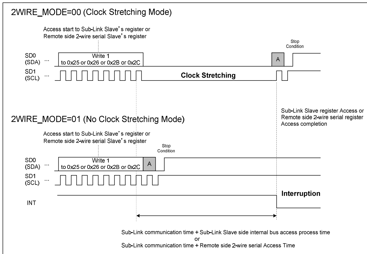
Figure 8. 2WIRE_MODE Operation
