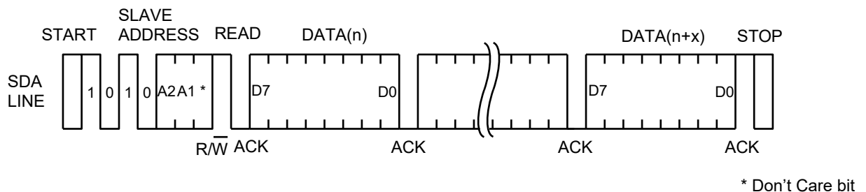
Figure 45. Sequential Read (in the Case of Current Read)
