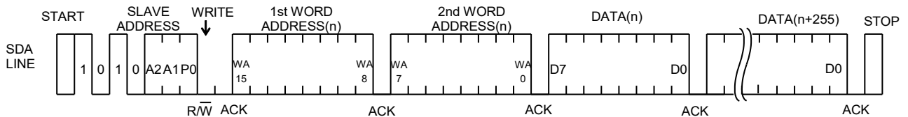
Figure 41. Page Write
