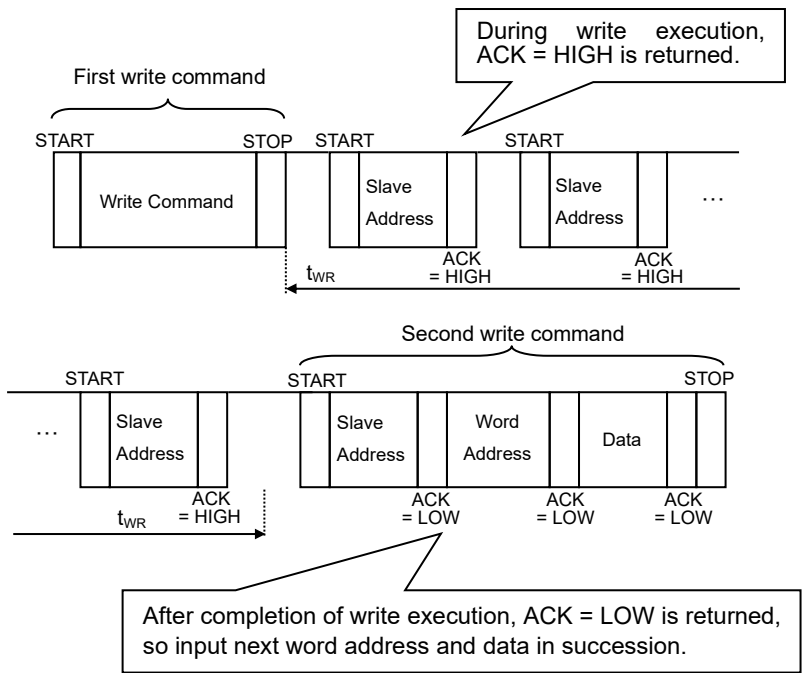
Figure 47. The Case of Continuous Write by Acknowledge Polling
