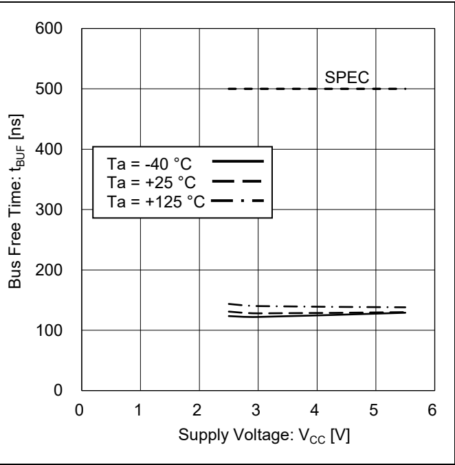
Figure 30. Bus Free Time vs Supply Voltage
