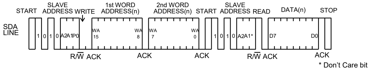
Figure 43. Random Read
