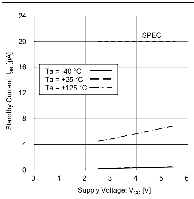
Figure 14. Standby Current vs Supply Voltage
