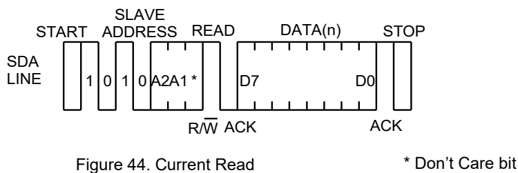
Figure 44. Current Read
