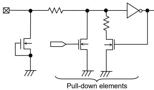
Figure 57. Input Pin Circuit Diagram (A1, A2, WP)
