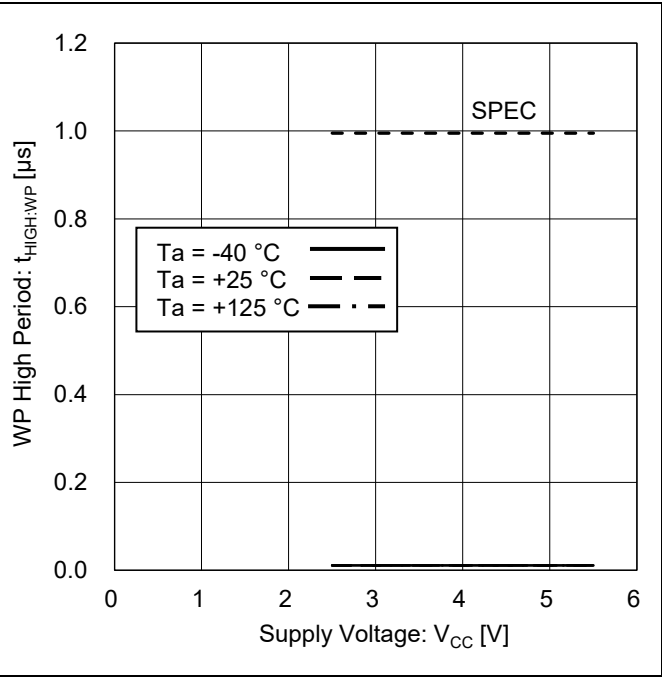
Figure 38. WP High Period vs Supply Voltage
