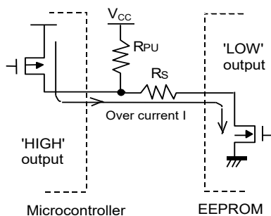
Figure 54. I/O Circuit Diagram
