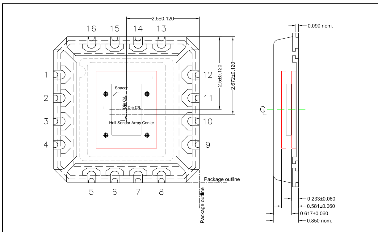
Figure 15: Hall element positions
