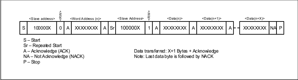
Figure 8: Data read with address pointer reload (Slave Transmitter Mode)
