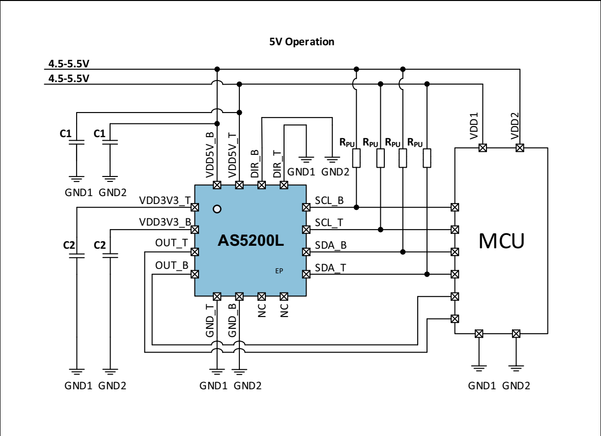
Figure 13: Application diagram for angle readout and programming with I²C
