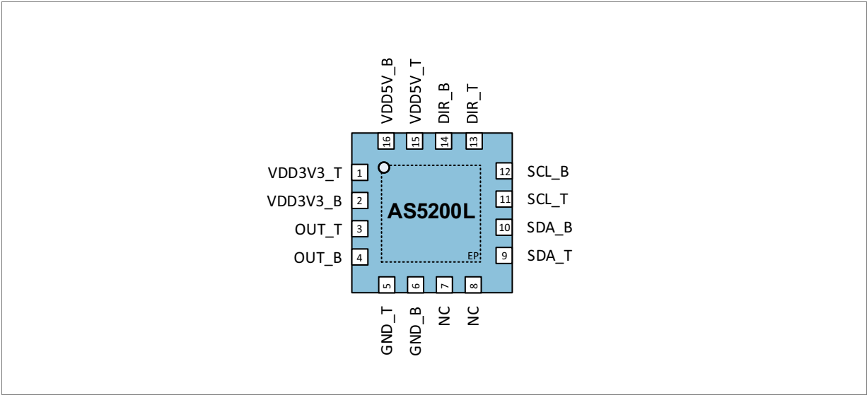
Figure 2: MLF-16 pin-out
