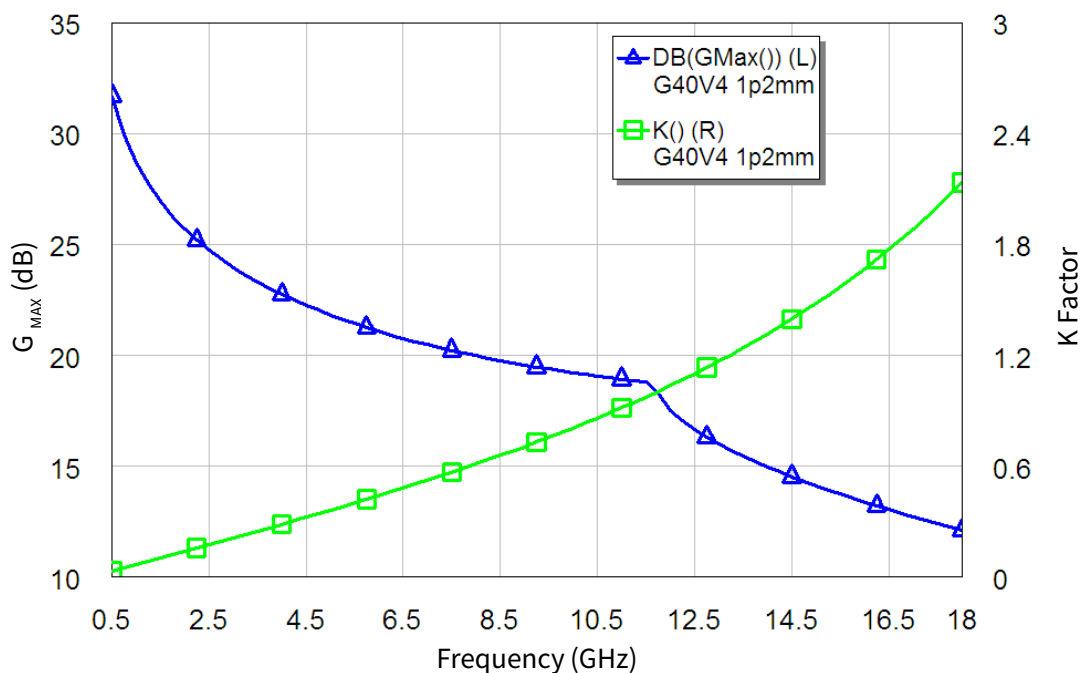
Figure 2. CGHV1J006D - Stability with G MAX and K Factor V DD = 40 V, I DS = 60 mA
