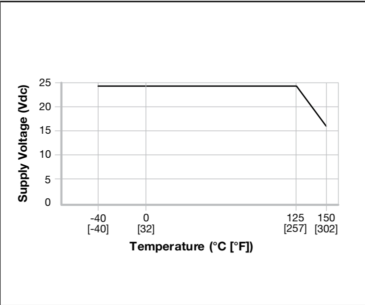
Figure 3. SS361RT Rated Supply Voltage
