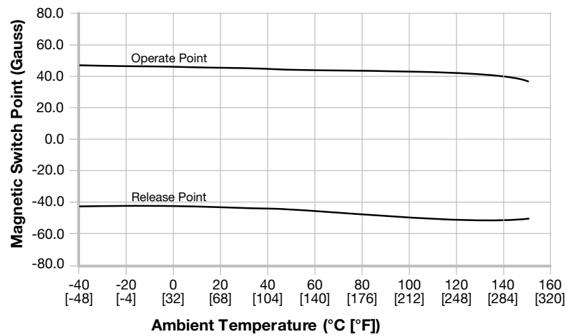
Figure 1. Typical Magnetic Characteristics vs Ambient Temperature at V_{\text{supply}} = 12 \text{ Vdc} .
