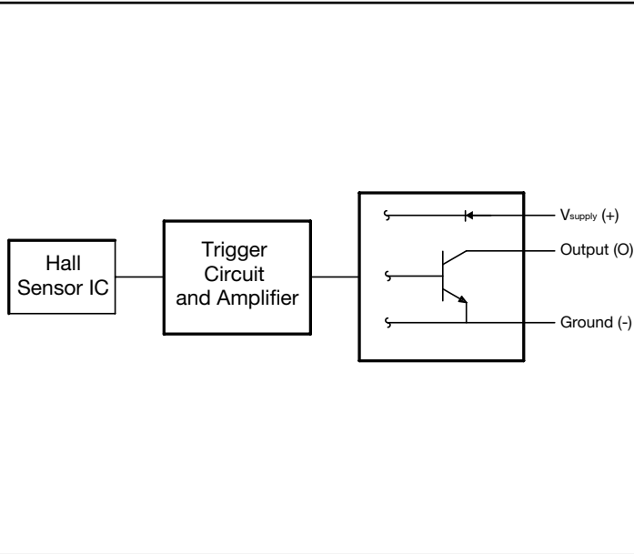
Figure 4. Magnetic Activation
