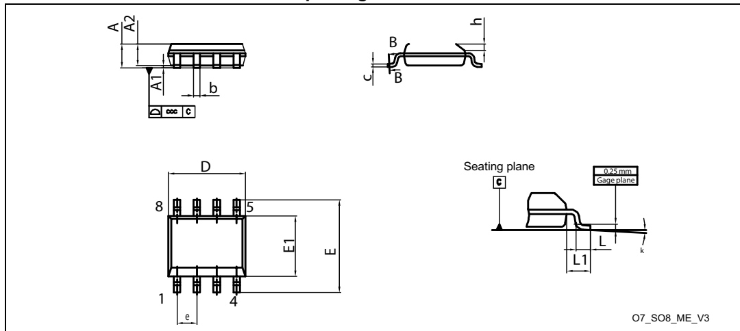
Figure 13. SO8 narrow – 8 lead plastic small outline, 150 mils body width, package outline
