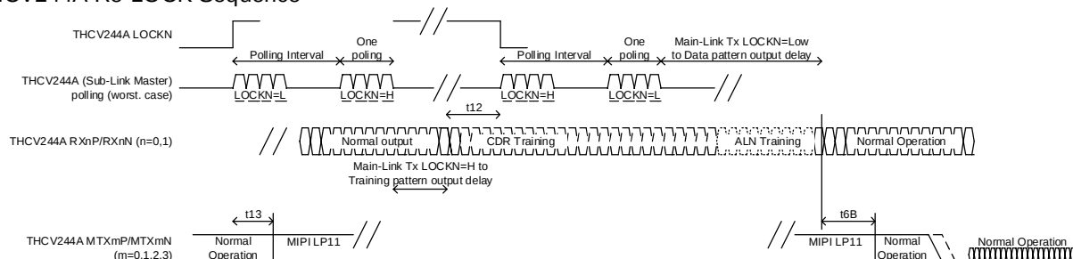
Figure 18. Re-Lock Sequence
