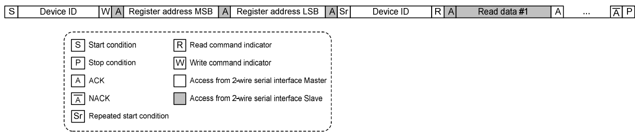
Figure 8. 2-wire serial I/F read to THCV244A local register protocol
