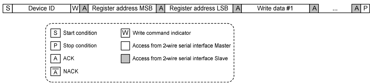
Figure 7. 2-wire serial I/F write to THCV244A local register protocol
