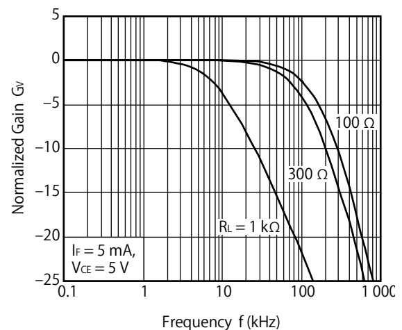
FREQUENCY RESPONSE
