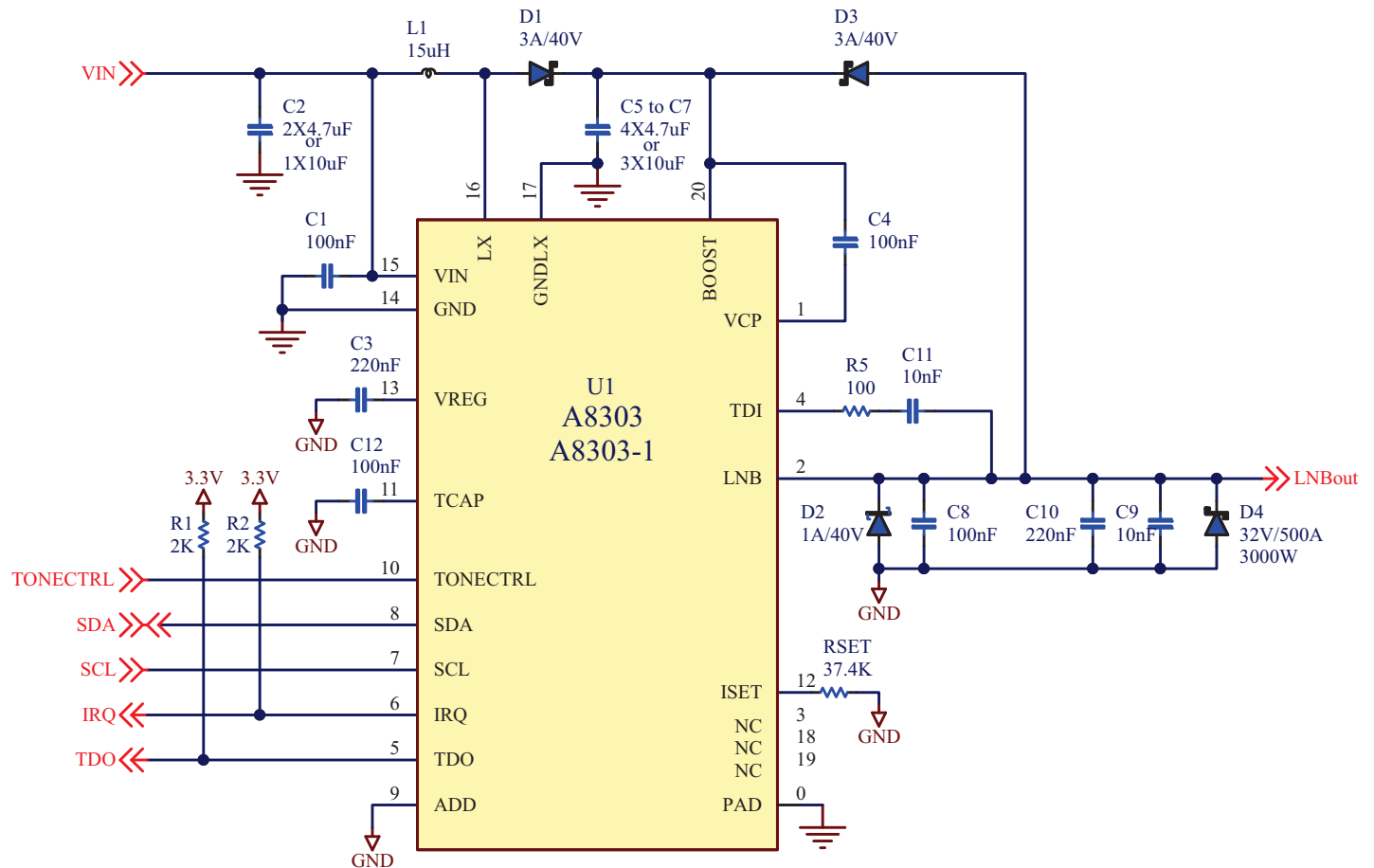
Schematic 2. DiSEqC 1.0 Applications, 12 V_{IN} \pm 10\% , 700 \text{ mA } I_{OUT} , surge of \pm 1000 \text{ V} , 2 \Omega , 1.2/50 \mu\text{s} - 8/20 \mu\text{s} combination wave
