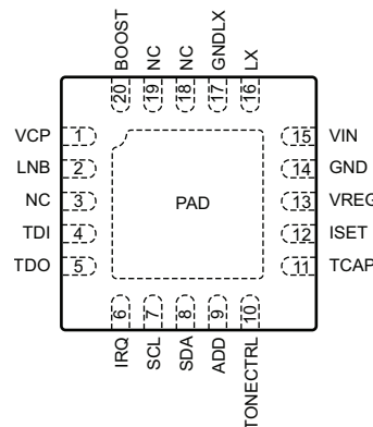
Pinout Diagram
