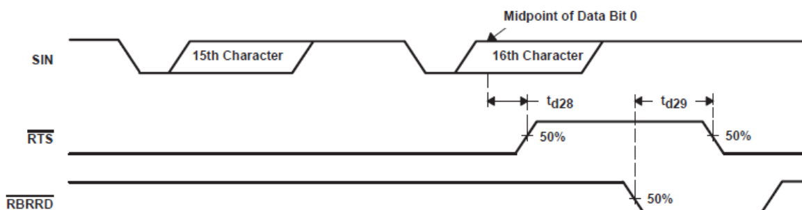
Figure 6-15. Auto-RTS Timing for RCV Threshold of 14 Waveforms
