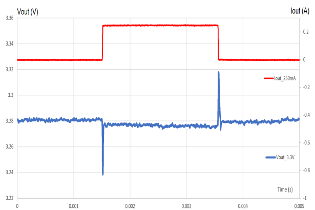
Figure 30. Maximum load variation response ( V_o = 3.3\text{ V} )
