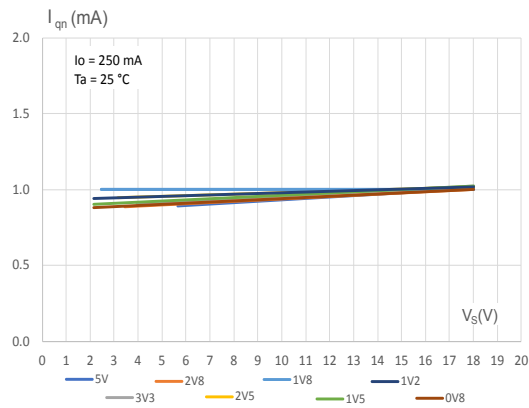
Figure 9. Current consumption vs input voltage ( I_o = 250 mA)
