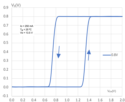
Figure 13. Output voltage vs enable voltage ( V_o = 0.8 V)
