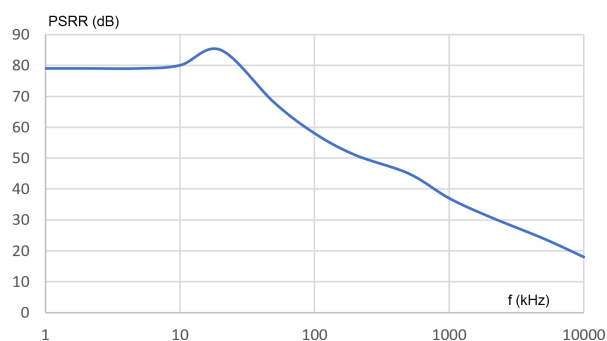
Figure 27. PSRR
