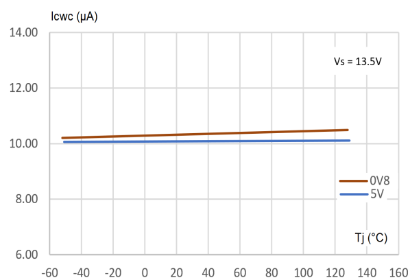
Figure 25. I_{cwc} vs T_j
