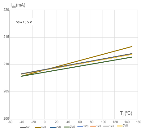
Figure 11. Short-circuit current vs T_j ( I_{short} pin floating)
