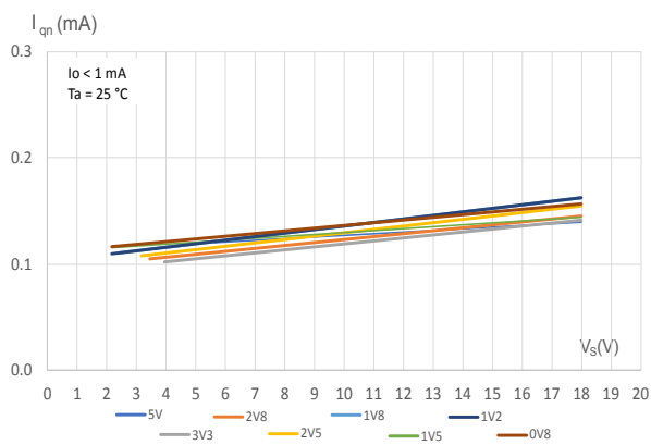
Figure 7. Current consumption vs input voltage ( I_o < 1 mA)
