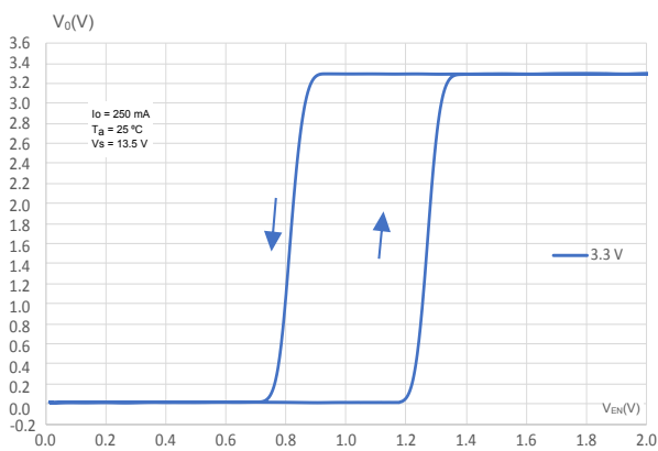
Figure 19. Output voltage vs enable voltage ( V_O = 3.3\text{ V} )
