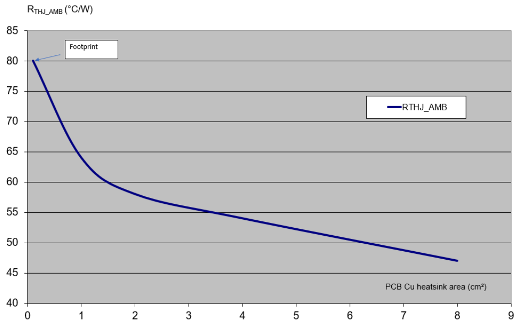
Figure 45. R_{thj-amb} versus PCB copper area in open box free air condition
