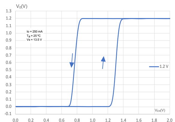
Figure 14. Output voltage vs enable voltage ( V_o = 1.2 V)
