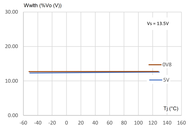
Figure 24. V_{wlth} vs T_j
