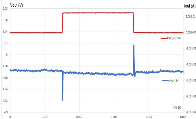
Figure 29. Maximum load variation response ( V_o = 5\text{ V} )
