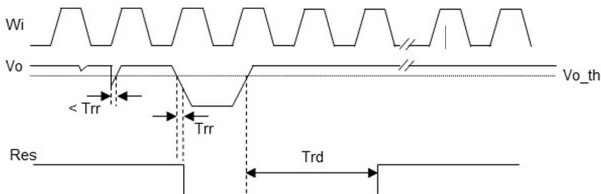
Figure 37. Reset timing diagram
