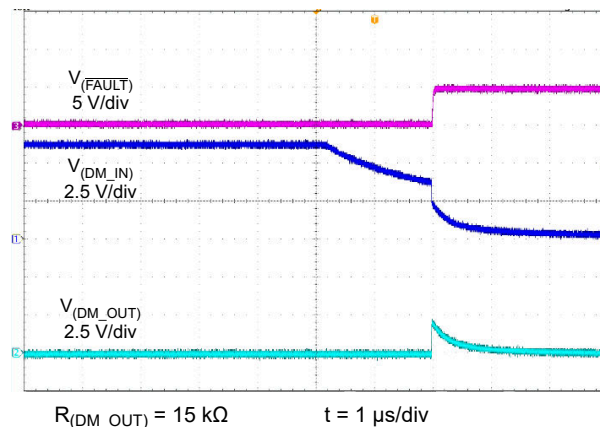
Figure 6-31. DM_IN Short-to- V_{BUS} Recovery
