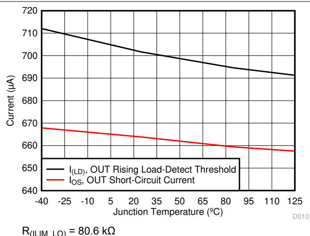
Figure 6-10. I_{OUT} Rising Load-Detect Threshold and OUT Short-Circuit Current Limit vs Temperature
