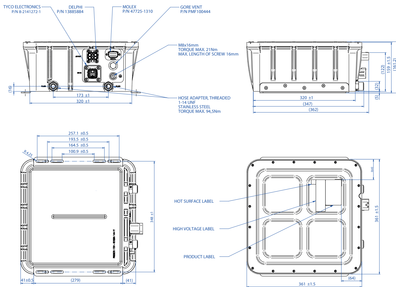
Figure 5. Front view
