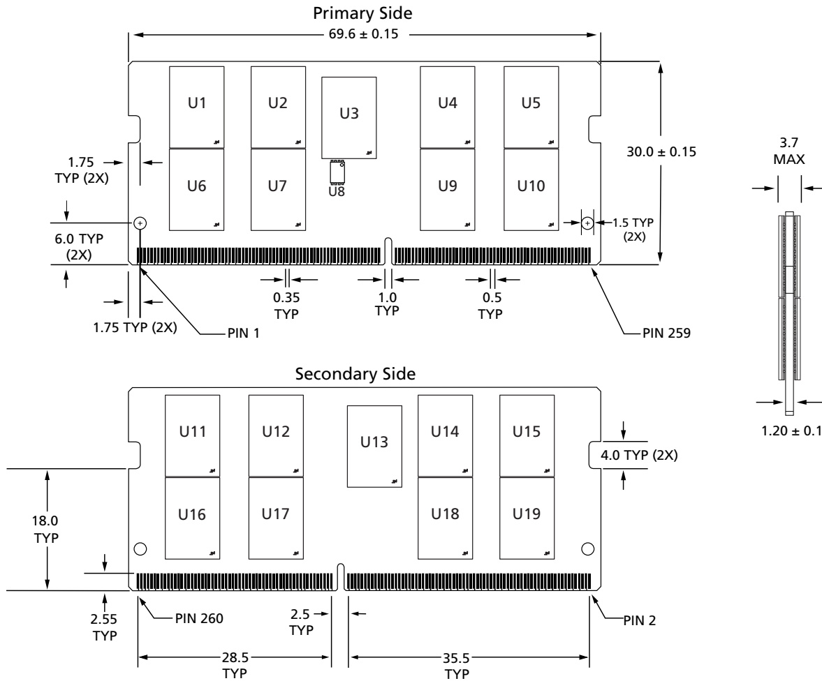
Figure 6: 260-Pin DDR4 SODIMM, PCB 2451 (R/C-G1)
