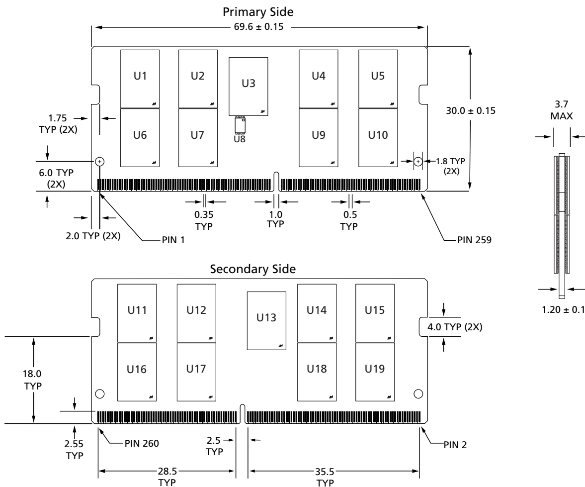
Figure 7: 260-Pin DDR4 SODIMM, PCB 3218,3240 (R/C-G1)
