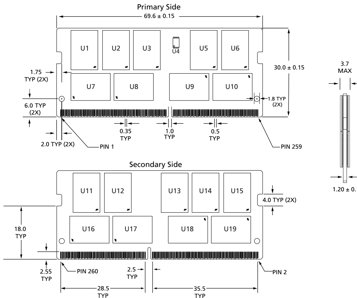
Figure 5: 260-Pin DDR4 SODIMM, PCB 1813 (R/C-H)
