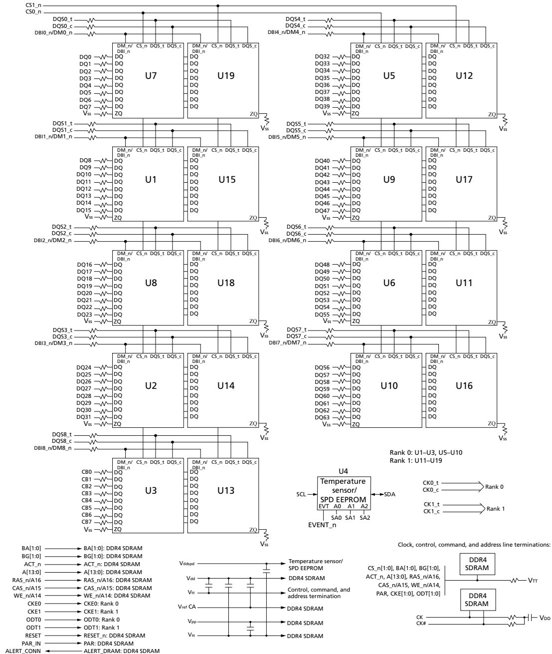
Figure 3: Functional Block Diagram, R/C-H (PCB 1813)
