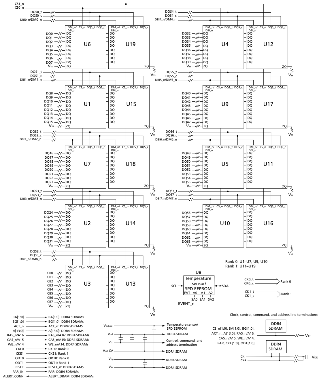
Figure 4: Functional Block Diagram, R/C-G1 (PCB 2451,3218,3240)
