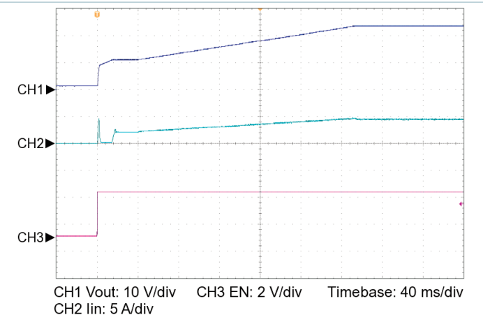
Figure 15 — Startup from EN, V_{IN} = 48\text{ V} , C_{OUT\_EXT} = 10000\text{ }\mu\text{F} , R_{LOAD} = 1.800\text{ }\Omega
