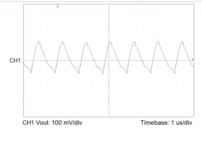
Figure 17 — Output voltage ripple, V_{IN} = 48\text{ V} , V_{OUT} = 24.0\text{ V} , C_{OUT\_EXT} = 1000\text{ }\mu\text{F} , R_{LOAD} = 1.800\text{ }\Omega
