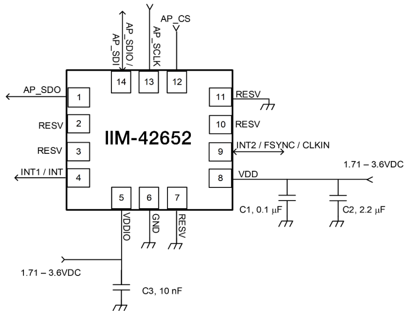
Figure 7. IIM-42652 Application Schematic (SPI Interface to Host)
