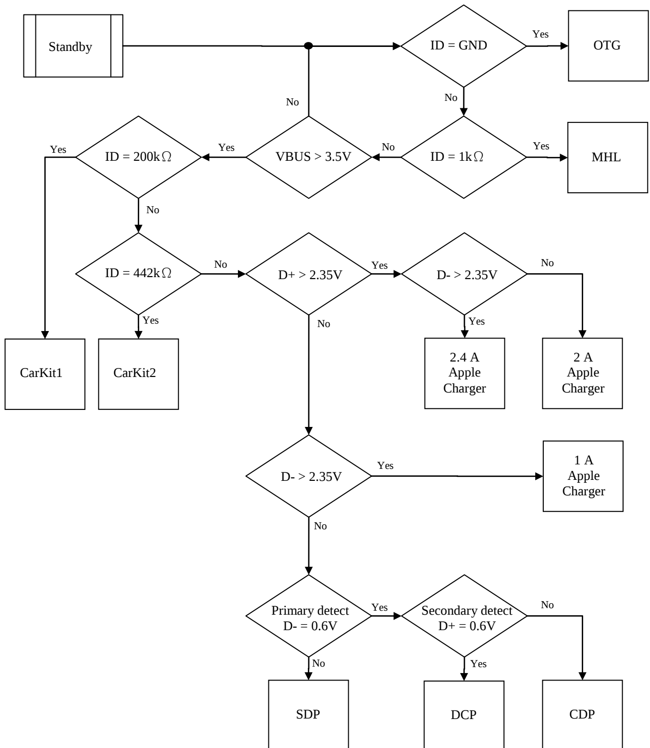
Figure 3. Accessory detection flowchart
