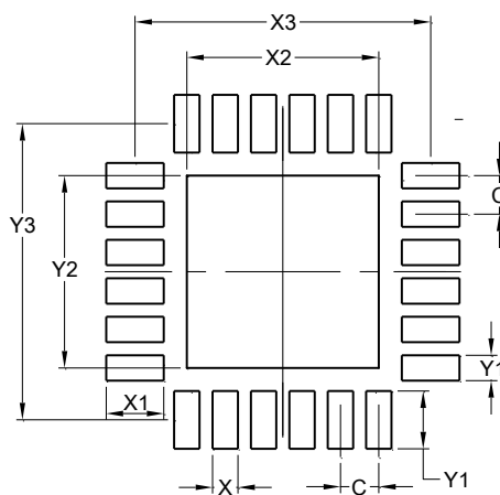
W-QFN4040-24/SWP (Type A1)
