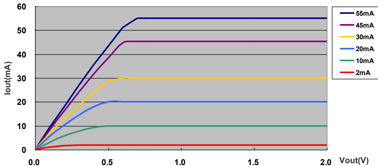
AL58263 IOUT vs. Vout Curve @ VDD=5V
