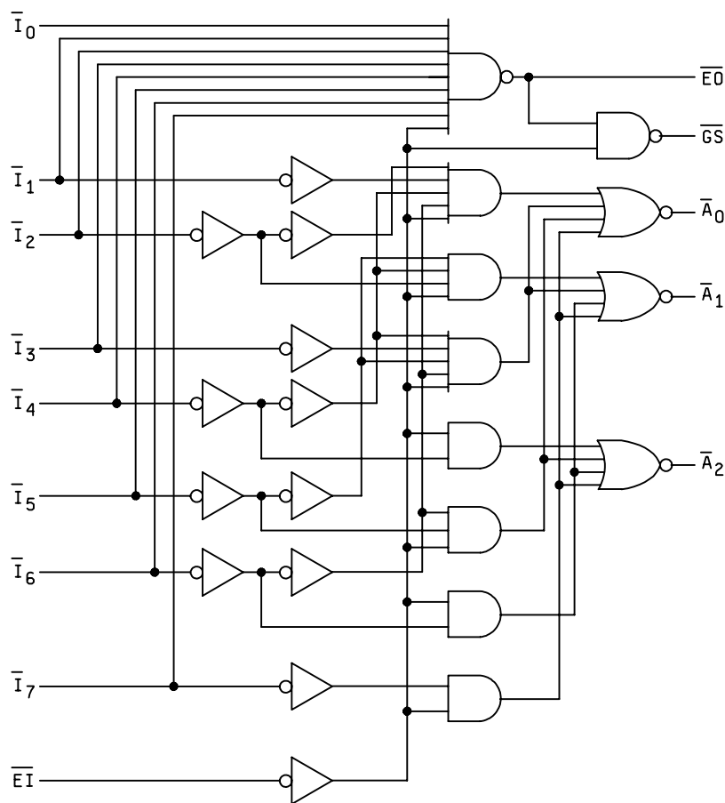
FIGURE 3. Logic diagram.
