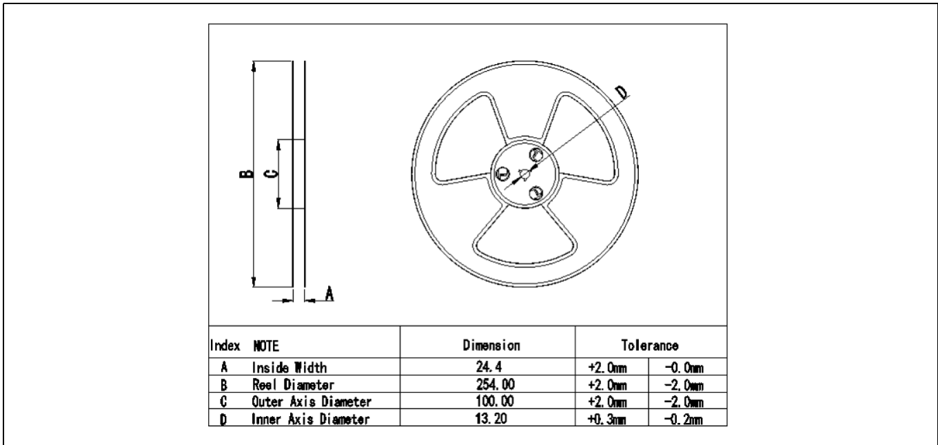
Figure 12 Reel dimensions
