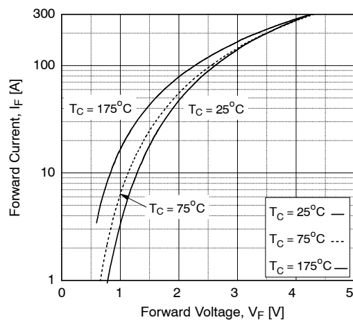
Figure 17. Forward Characteristics
