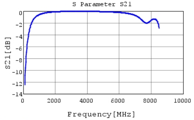
GRM1885C1H3R9CA01 S21 DCOV, 25degC
