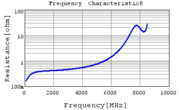
GRM1885C1H3R9CA01 R DCOV, 25degC
