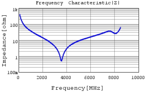
GRM1885C1H3R9CA01 |Z| DCOV, 25degC
