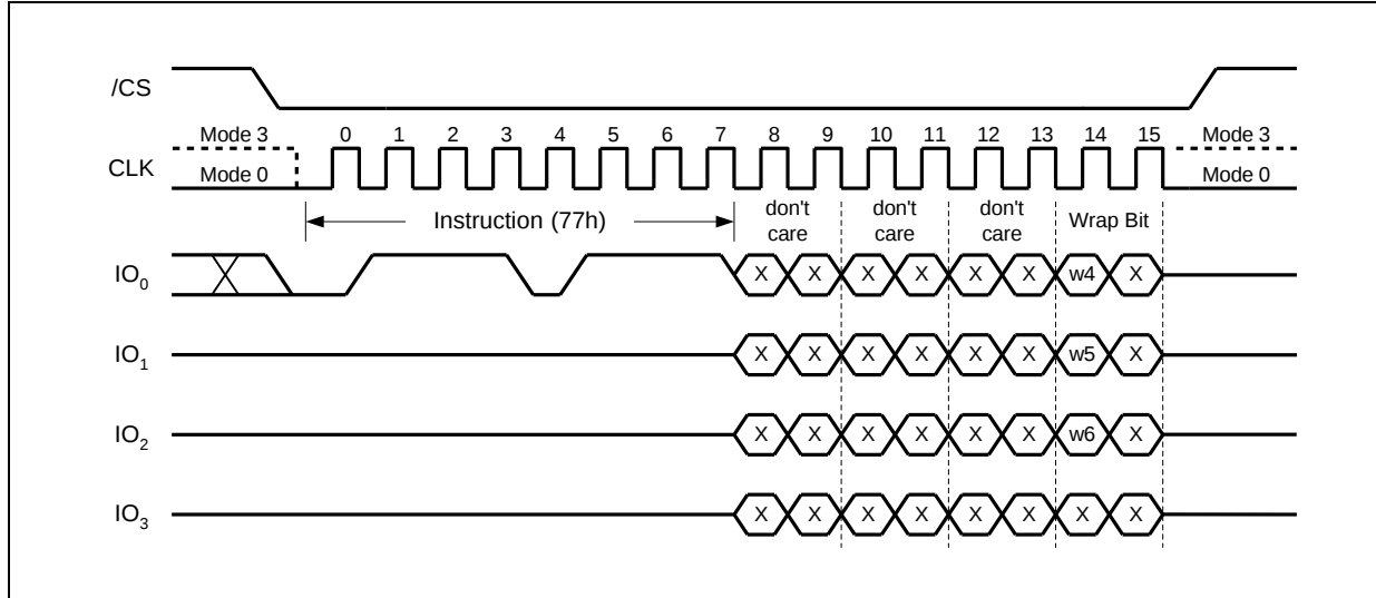
Figure 28. Set Burst with Wrap Command (SPI Mode only)
