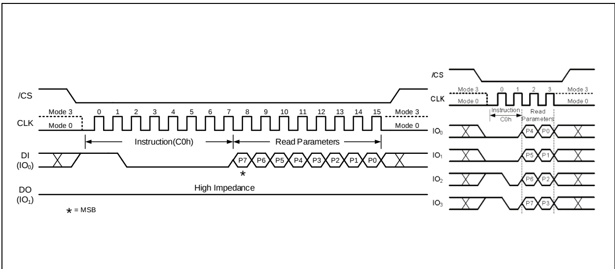
Figure 54. Set Read Parameters Command (SPI Mode Left/QPI Mode Right) "Set Read Parameters" command (C0h) can set the number of dummy clocks
