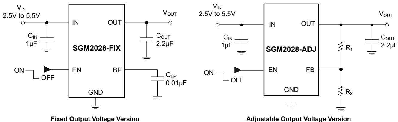
Figure 1. Typical Application Circuits
