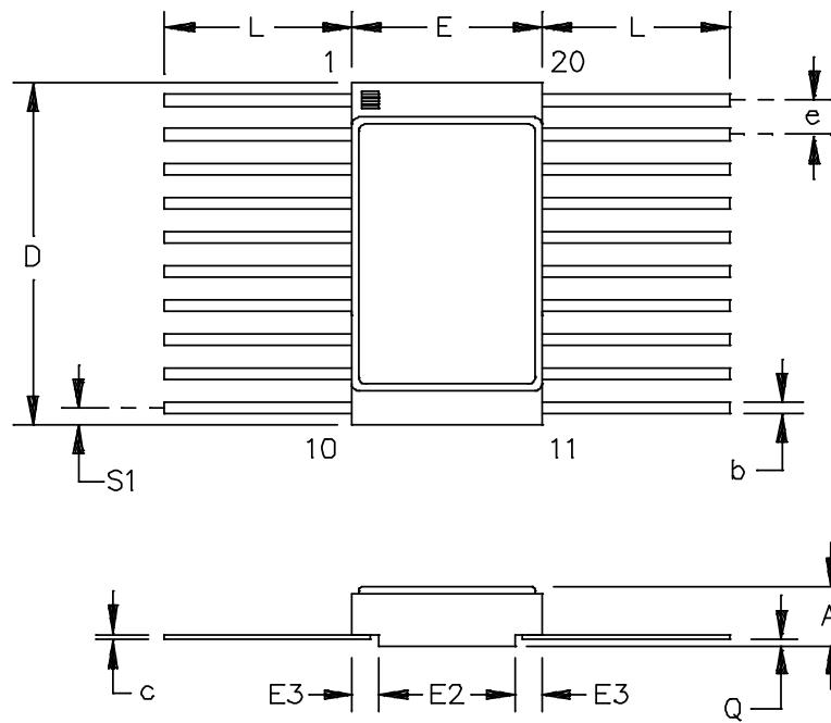
Case outline X and Y
