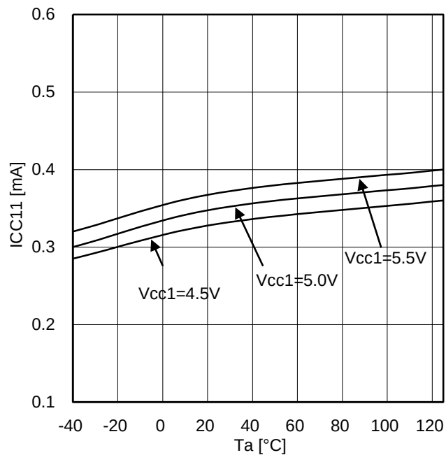
Figure 17. Input side circuit current (at OUT1=L )
