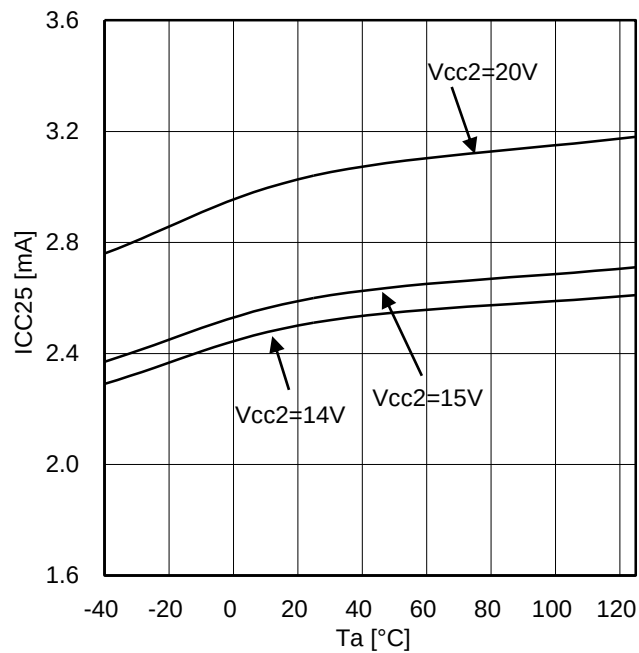
Figure 25. Output side circuit current (at OUT1=L )
