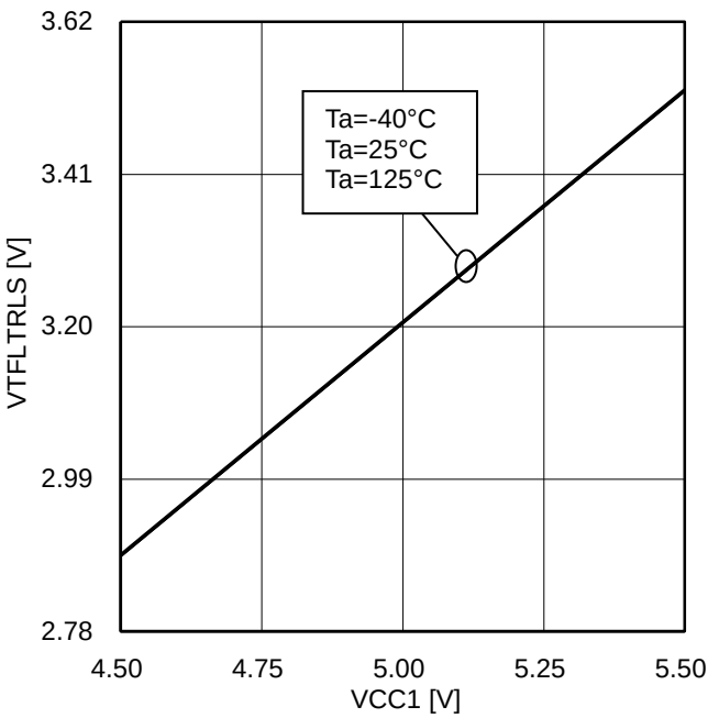
Figure 56. FLTRLS threshold
