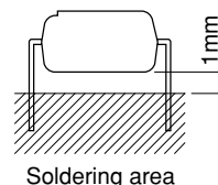
Soldering area
