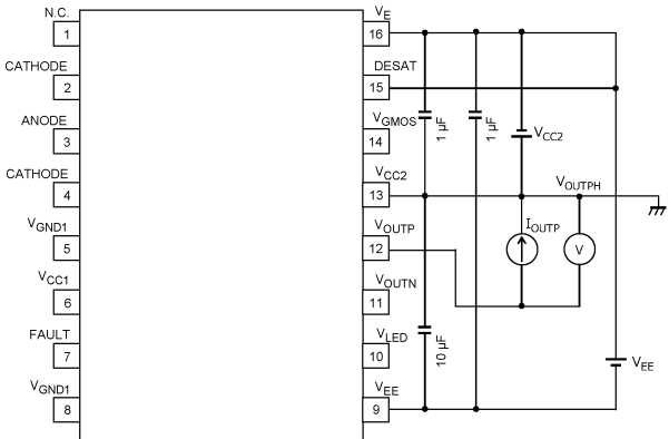
Fig. 13.1.5 V OUTPH , R OUTPH Test Circuit
