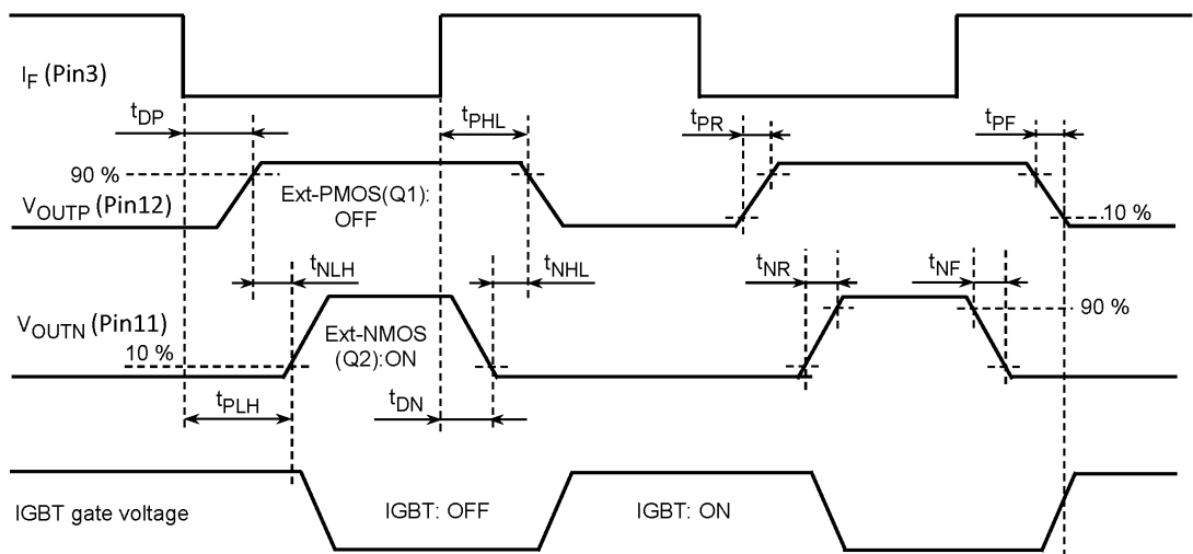
Fig. 13.2.1 Normal State
