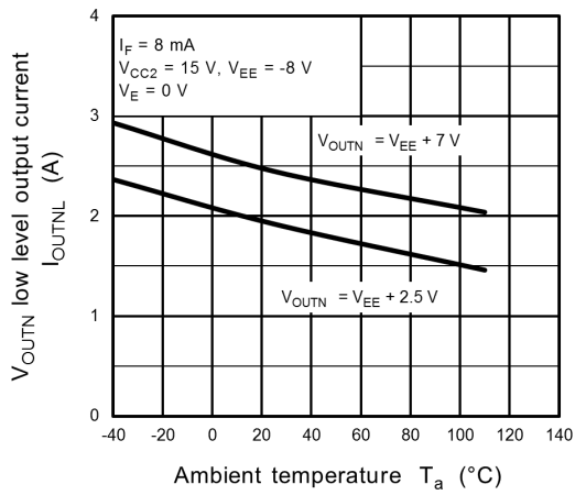
Fig. 13.3.6 I_{OUTNL} - T_a
