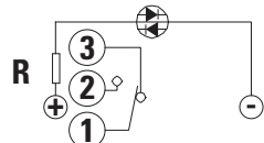
SPDT - Single Color LED
