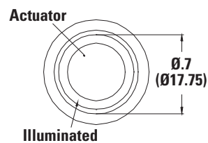
L7 & L8 Power & Ring
