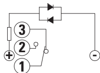
SPDT - Dual Color LED
