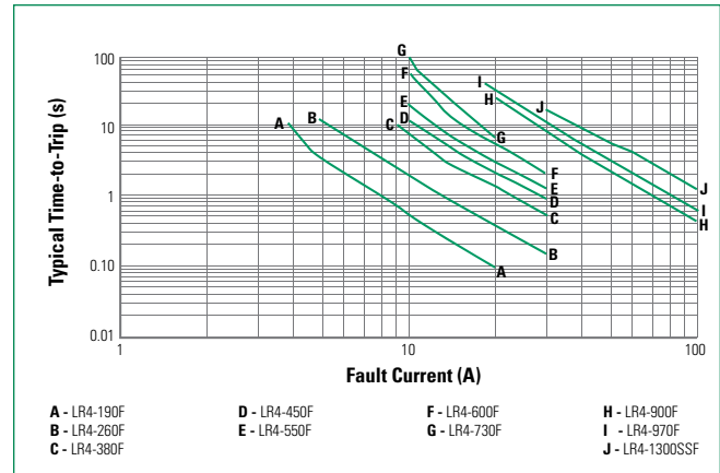
Typical Time-to-Trip Curve at 20°C
