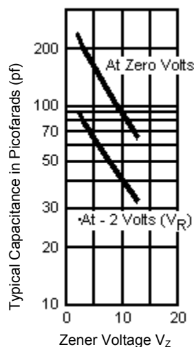
FIGURE 2 CAPACITANCE vs. ZENER VOLTAGE (TYPICAL)
