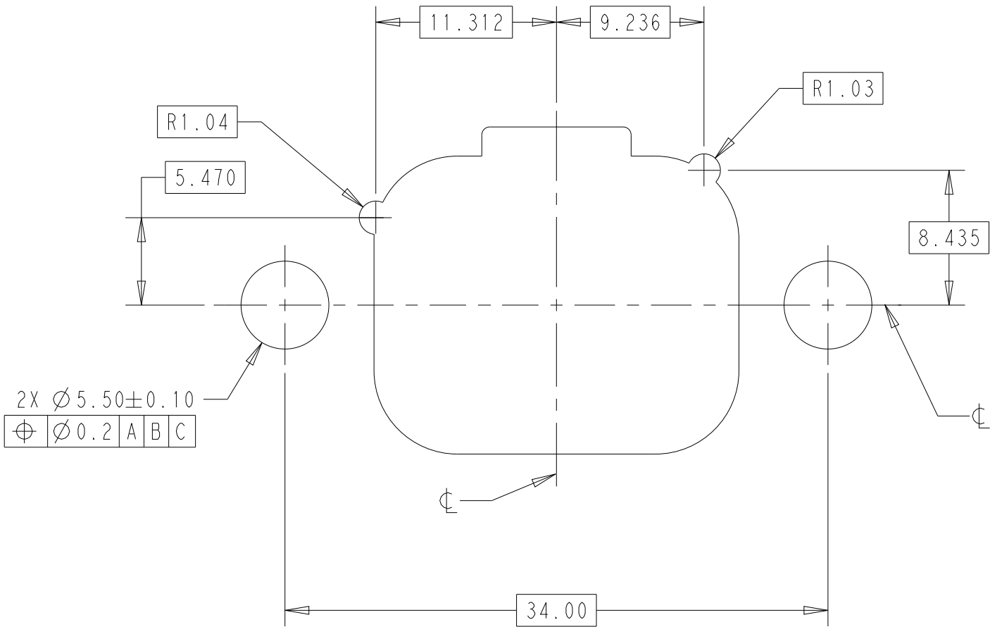
KEYWAY CLEARANCE DETAIL SCALE 3:1
