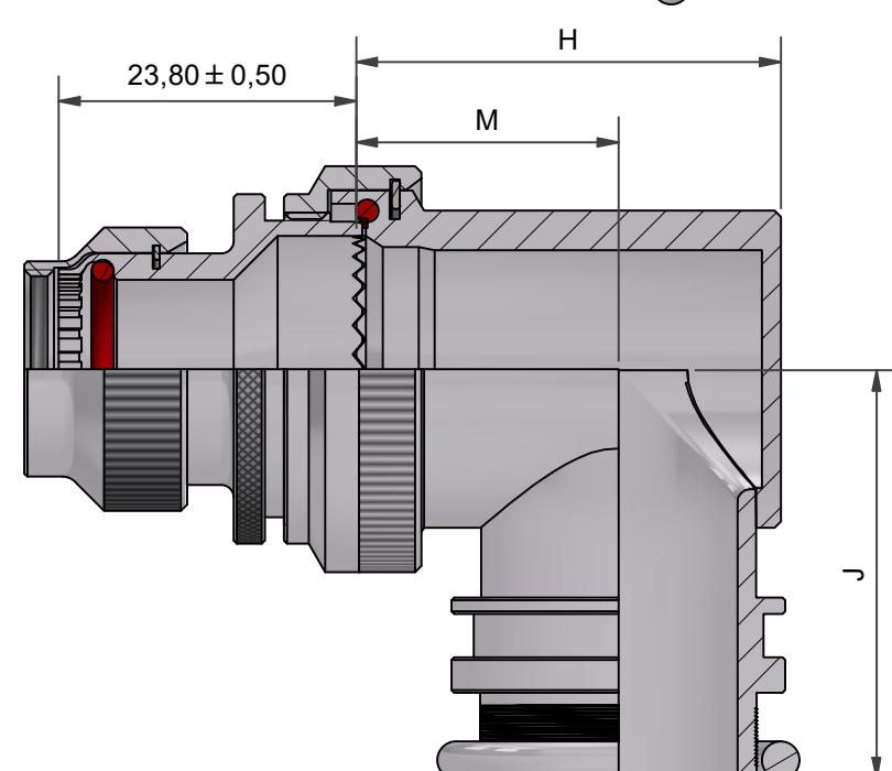
90° BACKSHELL - TYPE 2
