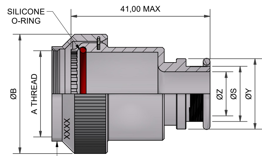
STRAIGHT BACKSHELL - TYPE 1
