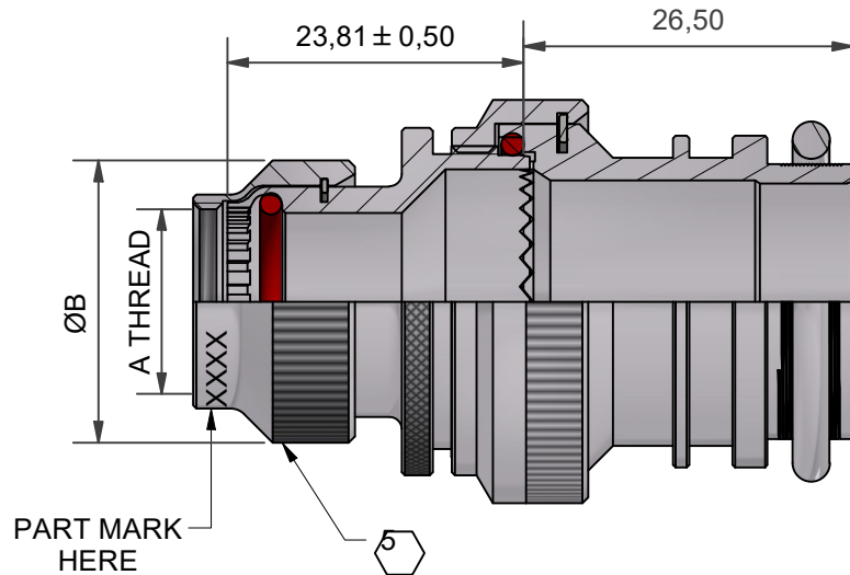
STRAIGHT BACKSHELL - TYPE 2
