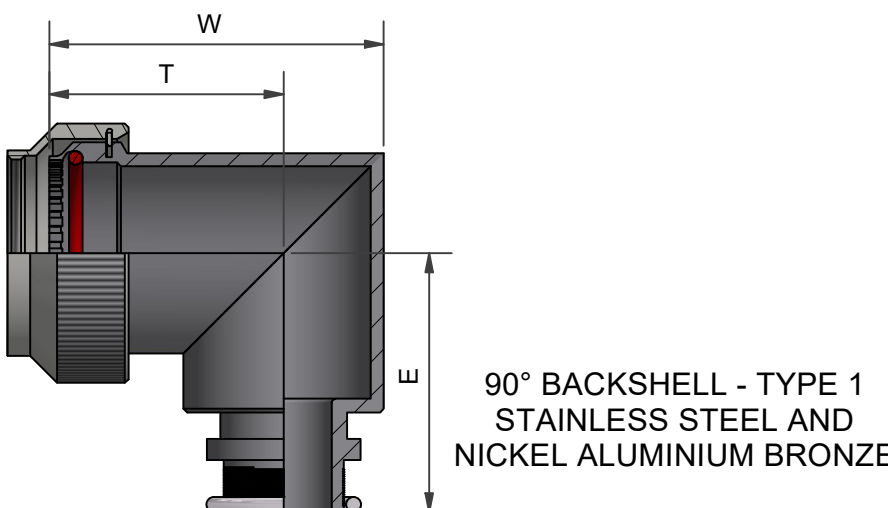
90° BACKSHELL - TYPE 1
