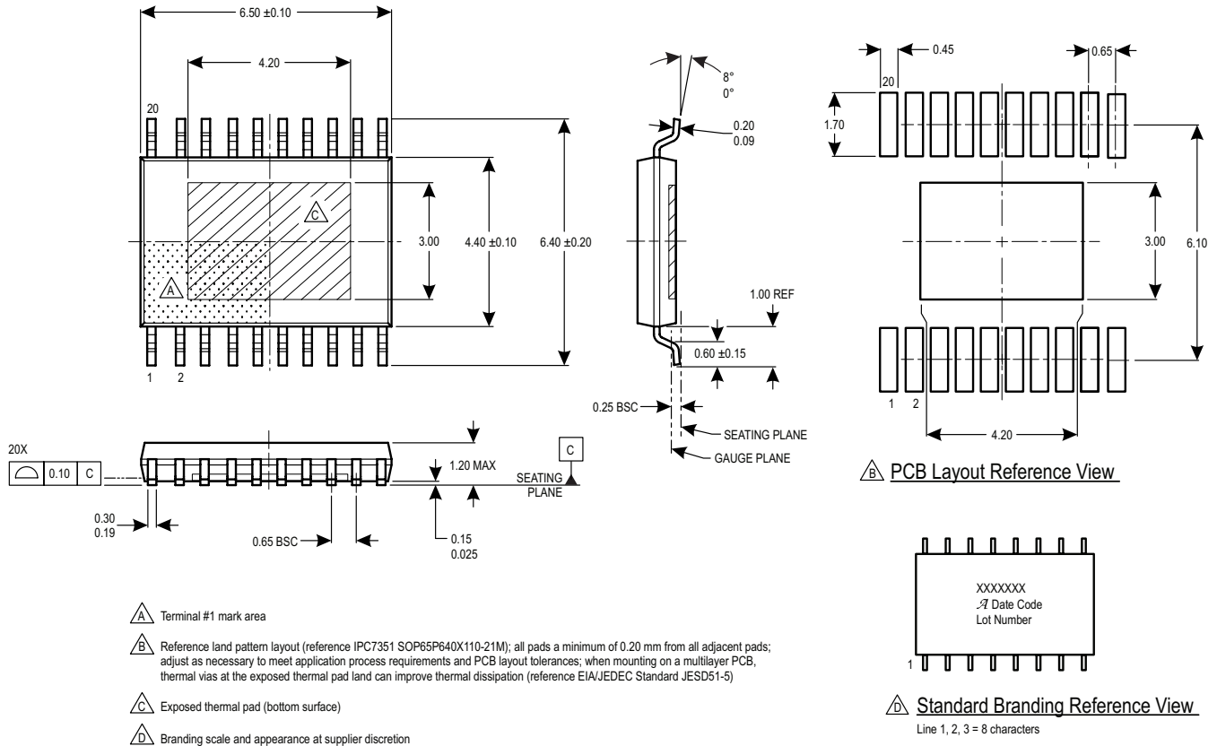
Figure 16: LP Package, 20-Pin TSSOP with Exposed Pad
