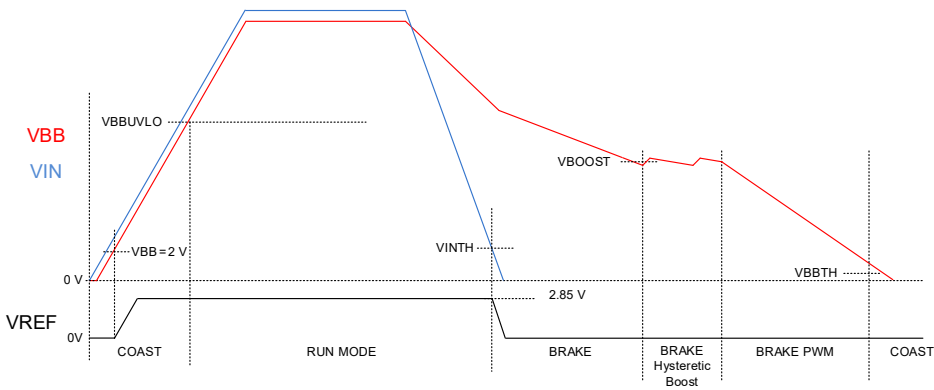
Figure 4: Normal Power Sequence
