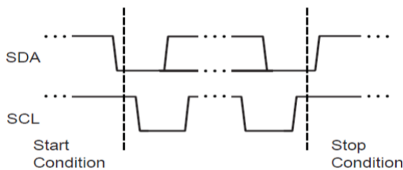
Figure 10: Start and Stop Conditions
