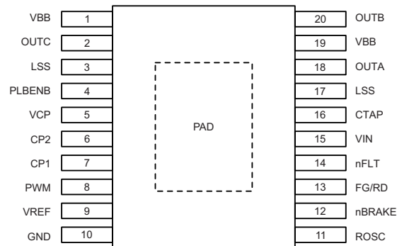
LP-20 Package Pinouts
