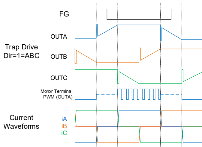
Figure 2: Trapezoidal Drive Sequence for DIR = HI
