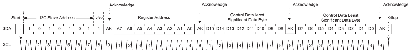
Figure 13: Write Command
