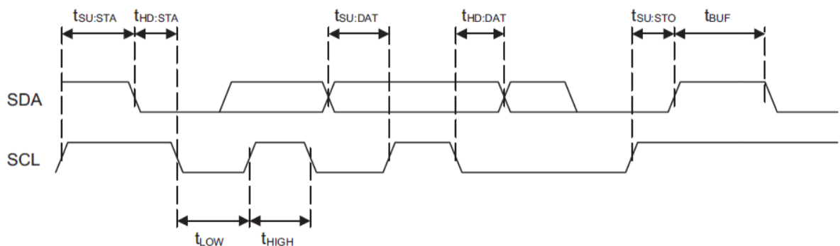
Figure 12: I 2 C-Compatible Timing Requirements
