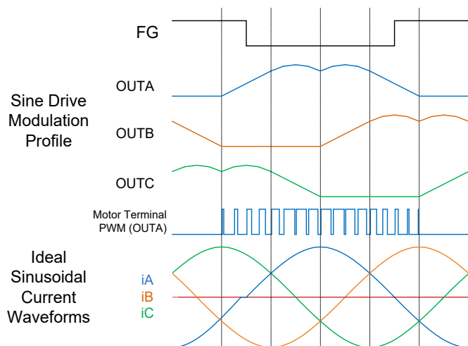
Figure 1: Sinusoidal Drive Sequence for DIR = HI
