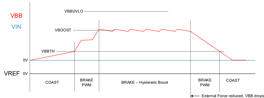
Figure 3: Motor spinning by external force, no power applied to fan module
