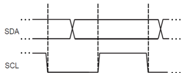
Figure 11: Clock and data bit synchronization
