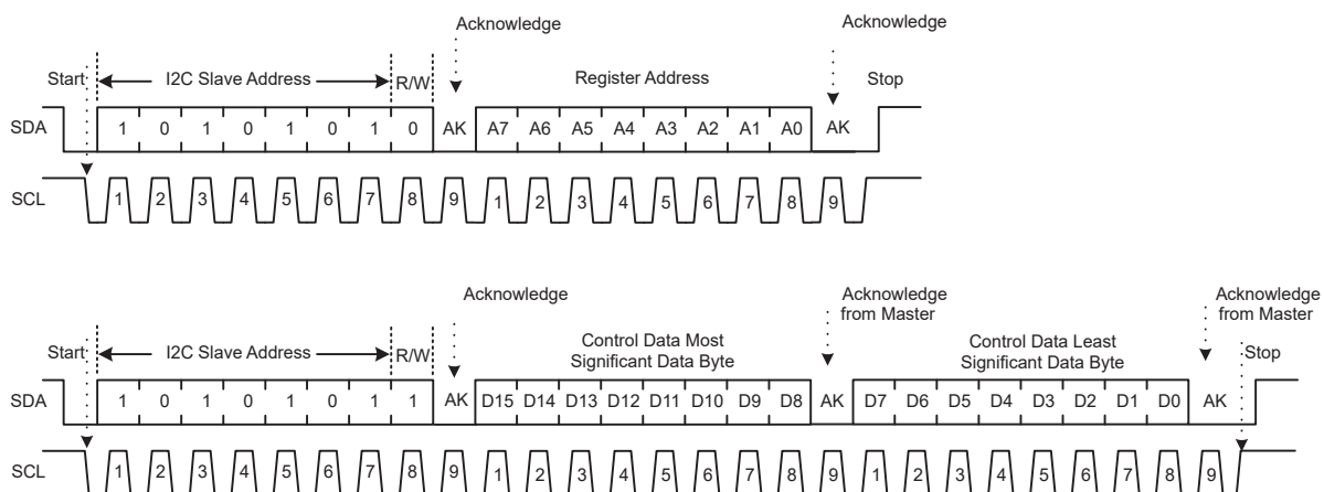
Figure 14: Read Command
