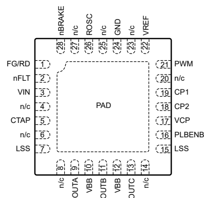
ET-28 Package Pinouts
