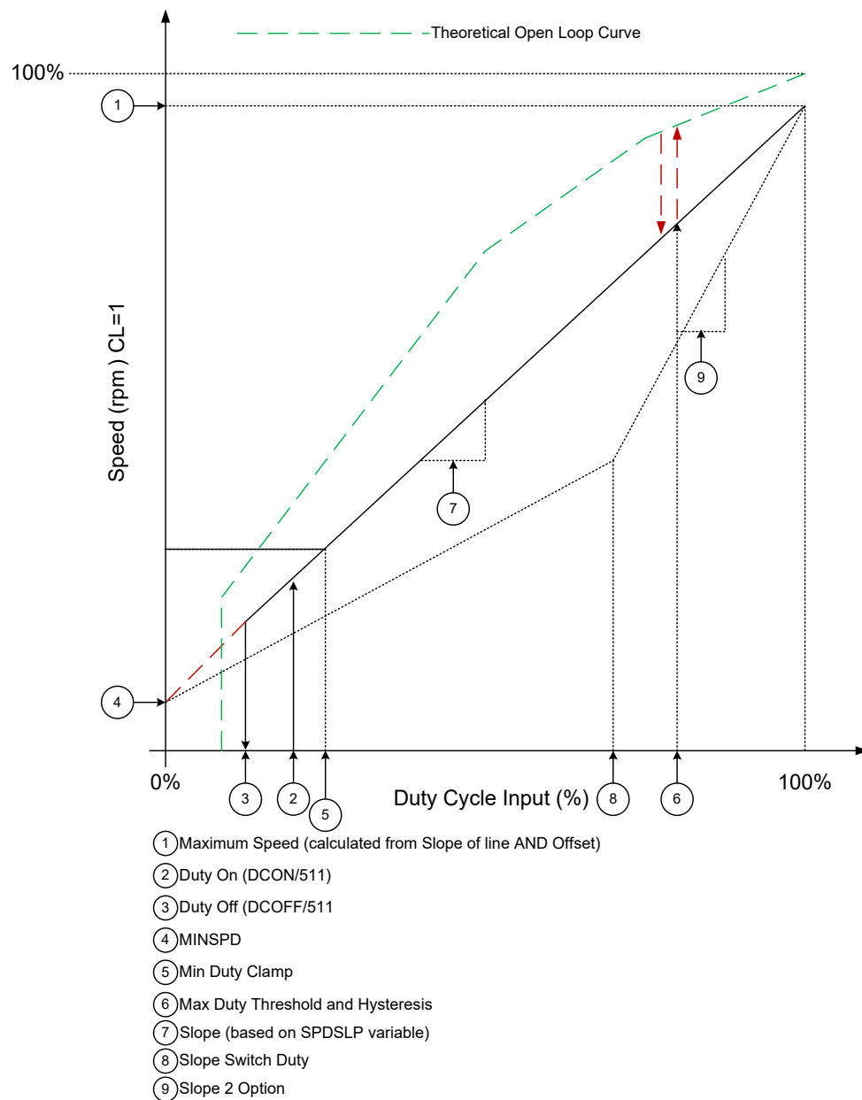
Figure 5: Speed Curve Parameters
