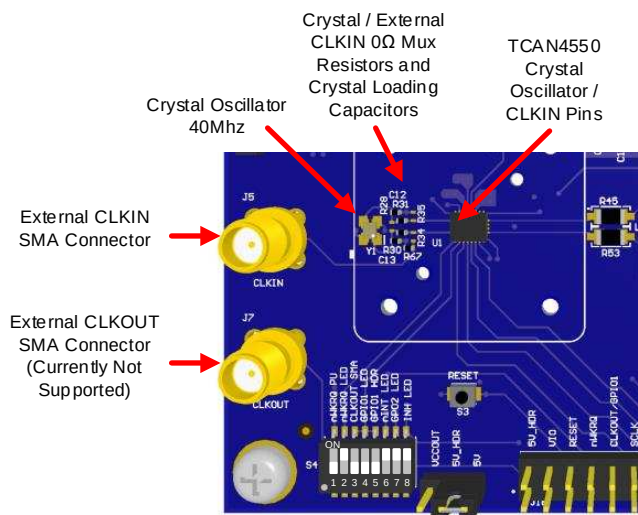
Figure 4. Clocking Features
