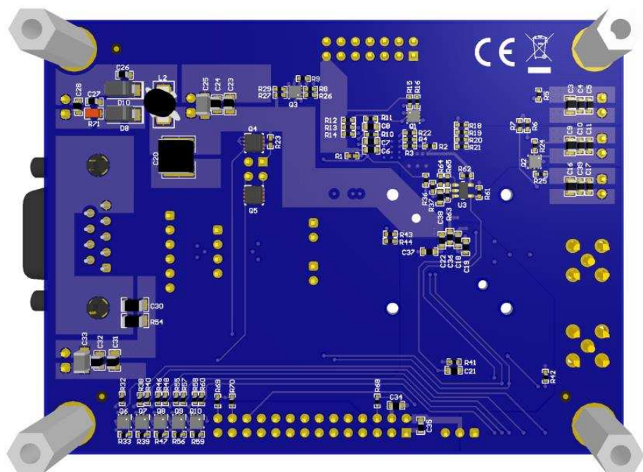
Figure 7. EVM Bottom
