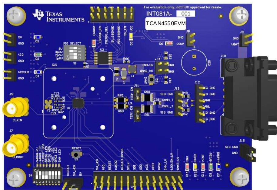
Figure 6. EVM Top
