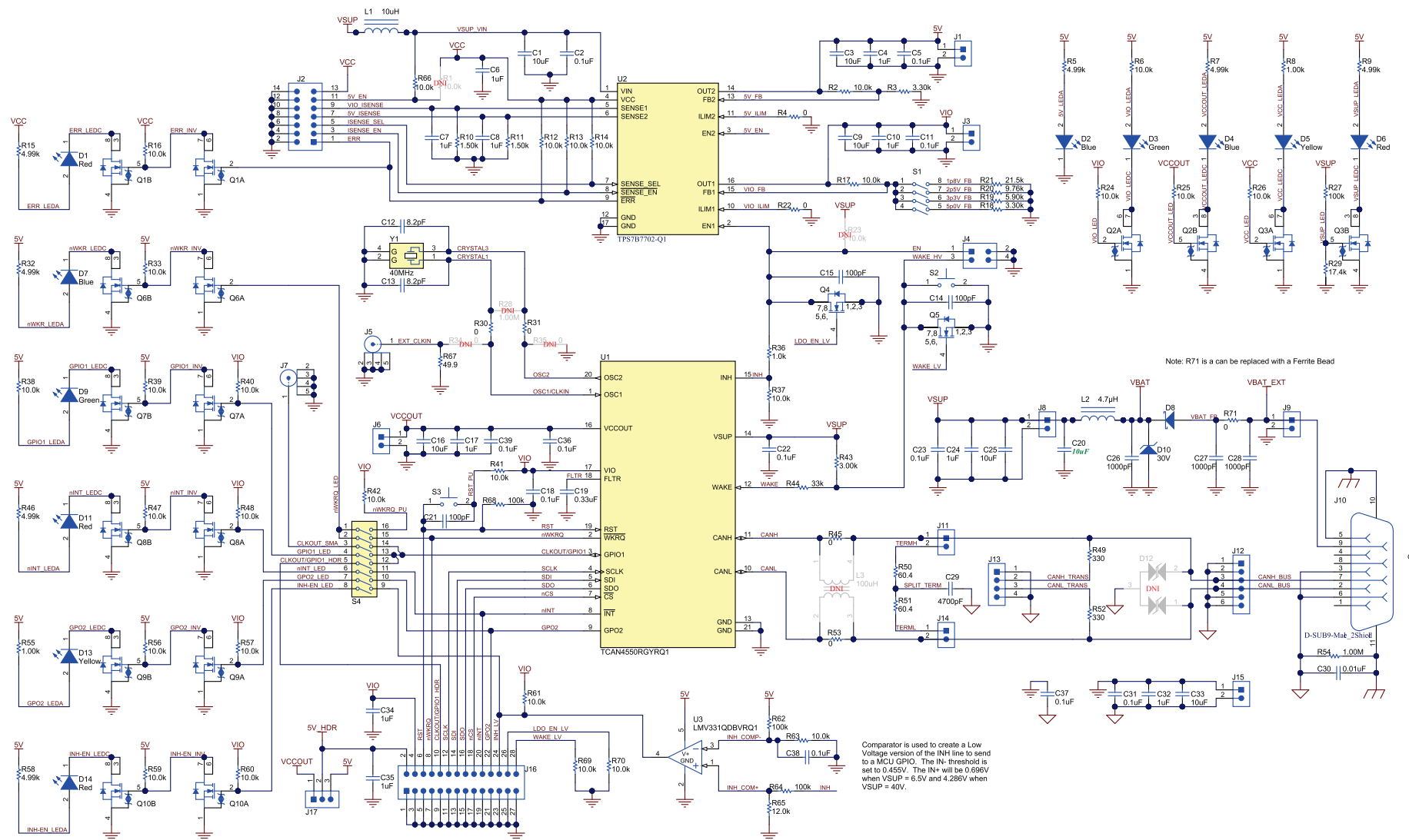
Figure 8. EVM Schematic
