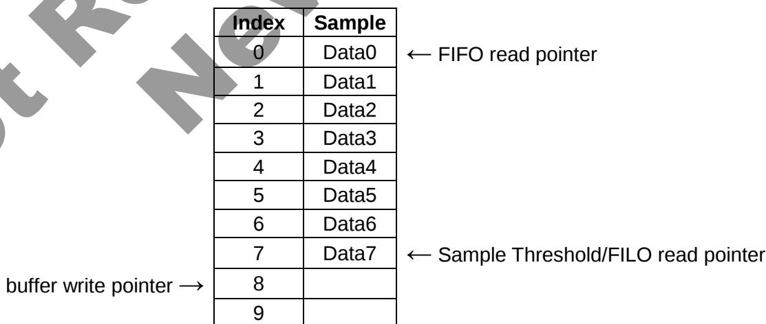
Figure 17: Buffer at Sample Threshold
