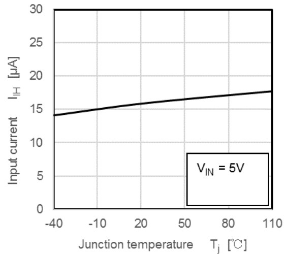
I_{IH} - T_j
