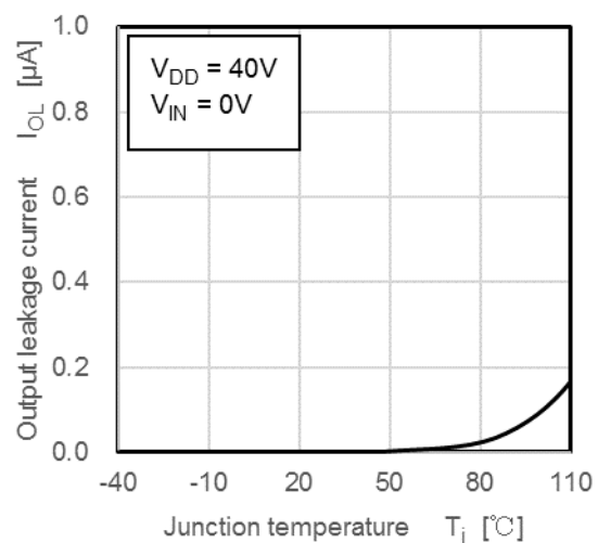
I_{OL} - T_j
