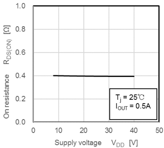
R_{DS(ON)} - V_{DD}
