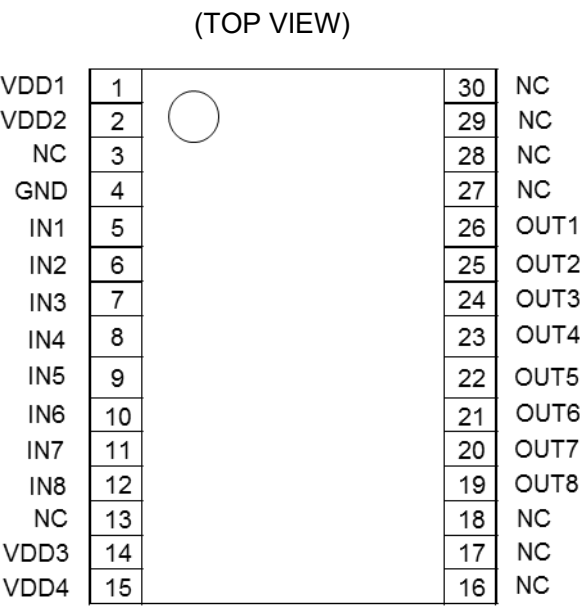
Figure 5.1 Pin Assignments
