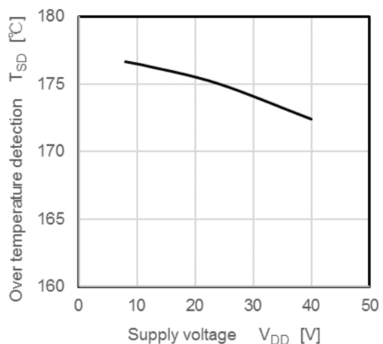
T_{SD} - V_{DD}
