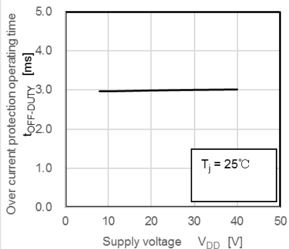
t_{OFF-DUTY} - V_{DD}
