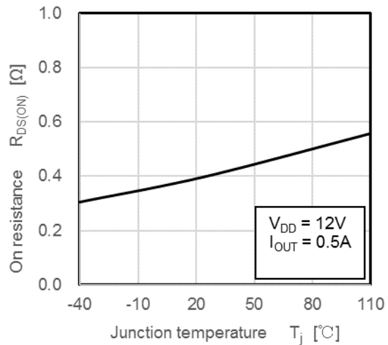
R_{DS(ON)} - T_j
