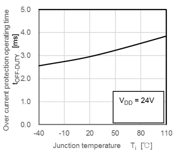
t_{OFF-DUTY} - T_j
