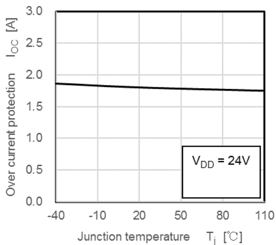
I_{OC} - T_j
