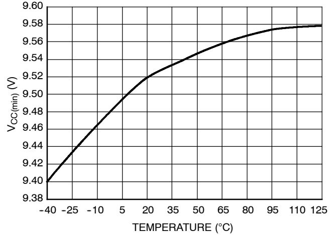
Figure 4. V CC(min)
