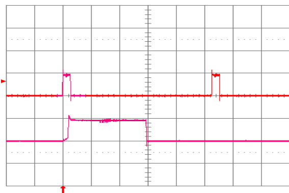
Fig. 1.8V.18: Load current (top trace, 20 \text{ A}/\text{div.} , 20 \text{ ms}/\text{div.} ) into a 10 \text{ m}\Omega short circuit during restart, at V_{in} = 24 \text{ V} . Bottom trace ( 20 \text{ A}/\text{div.} , 2 \text{ ms}/\text{div.} ) is an expansion of the on-time portion of the top trace.
