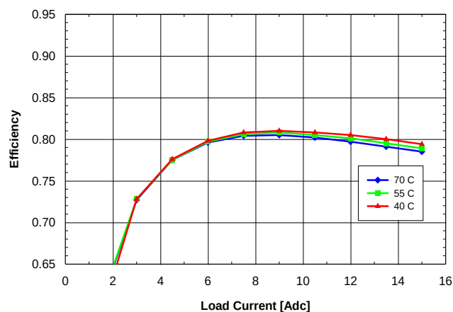
Fig. 1.0V.6: Efficiency vs. load current and ambient temperature for SQ24T/S15010 converter mounted vertically with V_{in} = 24V and air flowing from pin 3 to pin 1 at a rate of 200 LFM (1.0 m/s).
