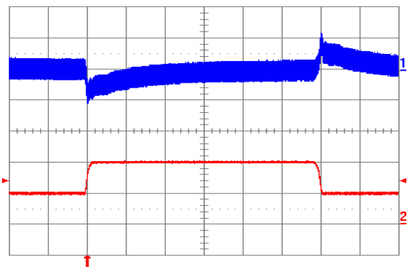
Fig. 6.0V.11: Output voltage response to load current step-change (2A - 4A - 2A) at V_{in} = 24\text{V} . Top trace: output voltage (100mV/div.). Bottom trace: load current (2A/div.). Current slew rate: 0.1 A/µs. C_o = 1\text{ }\mu\text{F} ceramic. Time scale: 0.2 ms/div.
