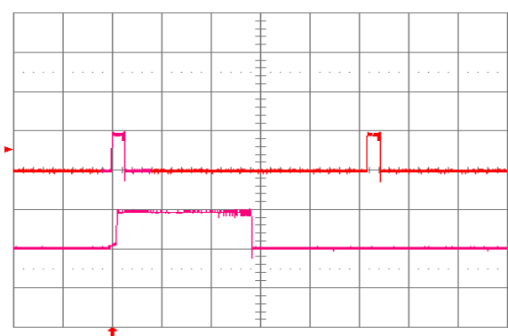
Fig. 2.0V.18: Load current (top trace, 20 \text{ A}/\text{div.} , 20 \text{ ms}/\text{div.} ) into a 10 \text{ m}\Omega short circuit during restart, at V_{in} = 24 \text{ V} . Bottom trace ( 20 \text{ A}/\text{div.} , 2 \text{ ms}/\text{div.} ) is an expansion of the on-time portion of the top trace.
