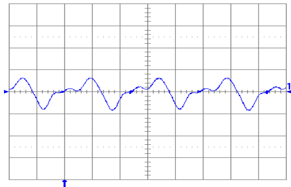
Fig. 1.8V.13: Output voltage ripple (20 mV/div.) at full rated load current into a resistive load with C_o = 10 \mu\text{F} tantalum + 1 \mu\text{F} ceramic and V_{in} = 24 \text{ V} . Time scale: 1 \mu\text{s}/\text{div} .
