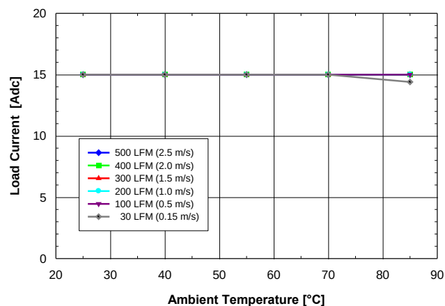
Fig. 1.8V.4: Available load current vs. ambient air temperature and airflow rates for SQ24S15018 converter mounted horizontally with V_{in} = 24V , air flowing from pin 3 to pin 1 and maximum FET temperature \leq 120^{\circ}C .
