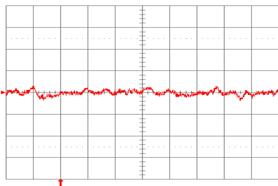
Fig. 1.8V.16: Input reflected ripple current, i_s (10 mA/div.), measured through 10 \mu\text{H} at the source at full rated load current and V_{in} = 24 \text{ V} . Refer to Fig. 1.8V.14 for test setup. Time scale: 1 \mu\text{s}/\text{div} .
