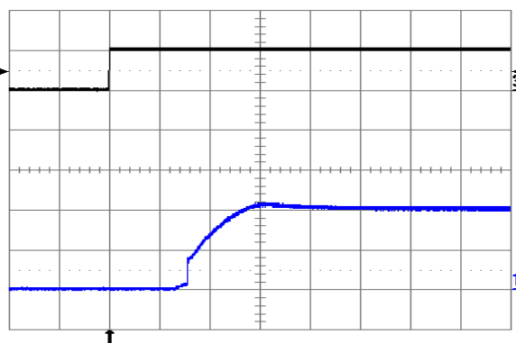
Fig. 1.0V.10: Turn-on transient at full rated load current (resistive) plus 10,000µF at V_{in} = 24\text{V} , triggered via ON/OFF pin. Top trace: ON/OFF signal (5 V/div.). Bottom trace: output voltage (0.5 V/div.). Time scale: 1 ms/div.
