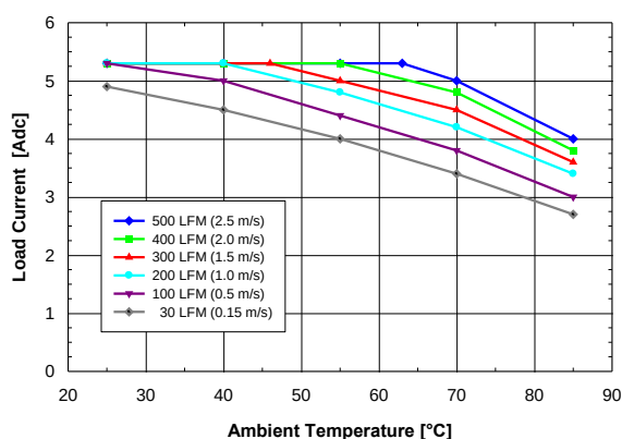
Fig. 8.0V.1: Available load current vs. ambient air temperature and airflow rates for SQ24T05080 converter with D height pins mounted vertically with V in = 24 V, air flowing from pin 3 to pin 1 and maximum FET temperature ≤ 120°C.
