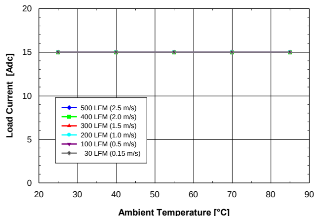
Fig. 1.0V.1: Available load current vs. ambient air temperature and airflow rates for SQ24T15010 converter with B height pins mounted vertically with V_{in} = 24V , air flowing from pin 3 to pin 1 and maximum FET temperature \leq 120^{\circ}C .
