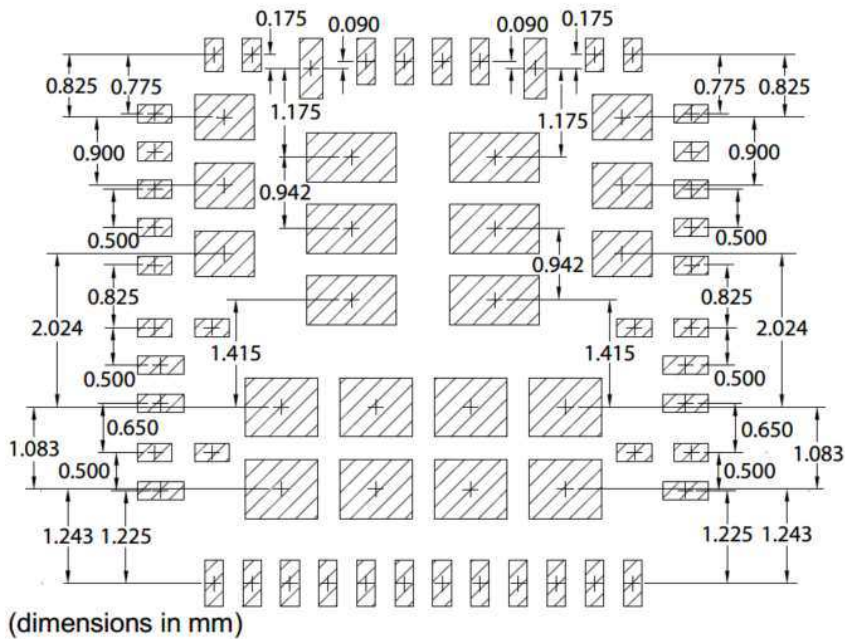
Figure 55 42-lead 7x7 stencil design_3
