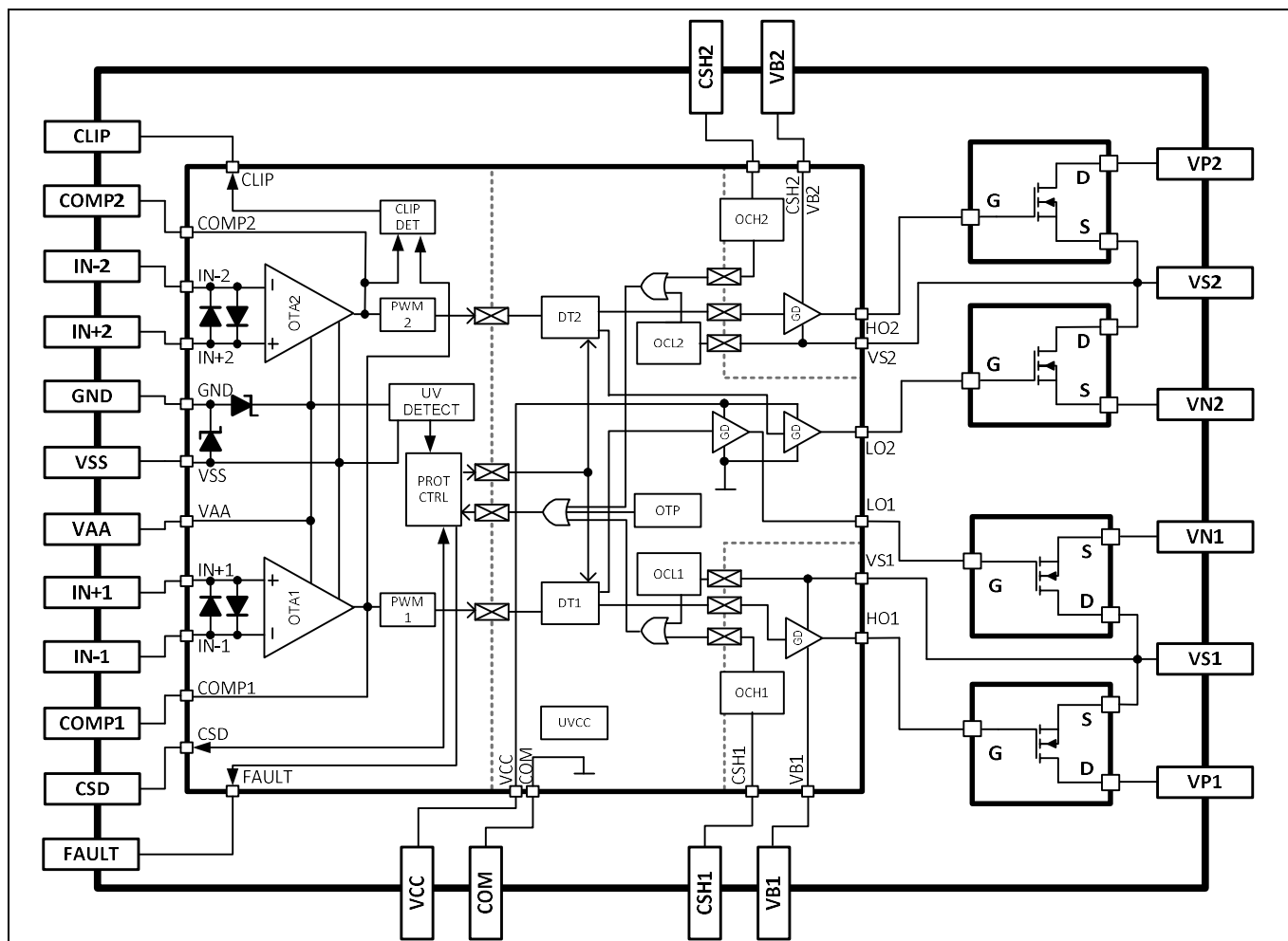
Figure 21 Block diagram
