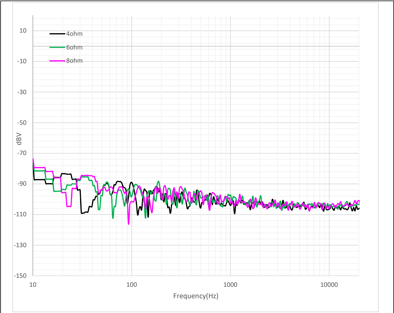
Figure 5 Noise floor
