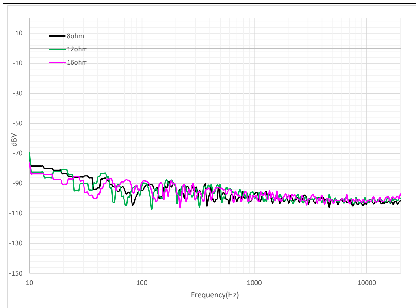
Figure 10 Noise floor
