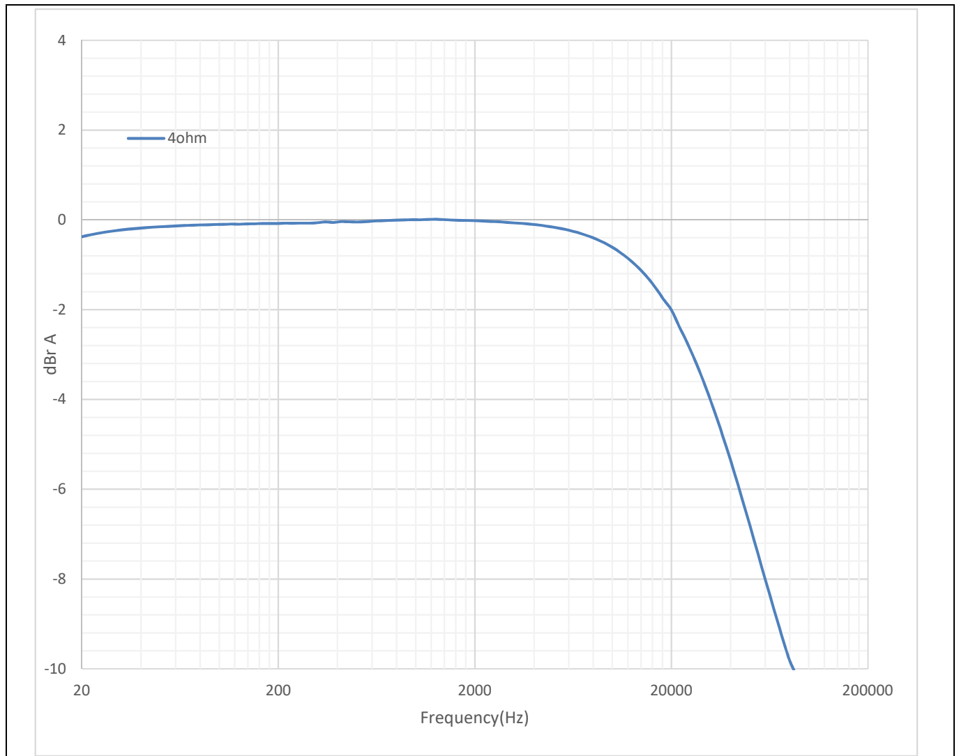
Figure 13 Frequency response
